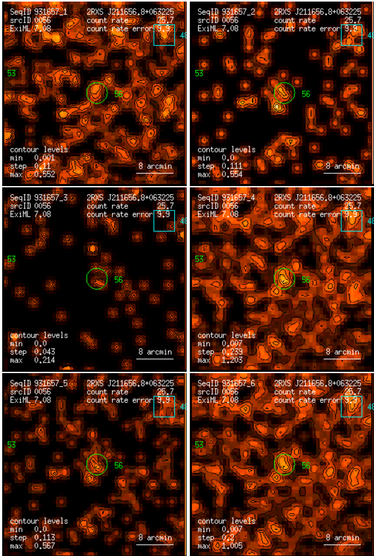
Figure 56: RASS 931657: detection 0056: band rate images, Gaussian filter: (1) PSPC channels 11 – 41, (2) 52 – 90, (3) 91 – 201, (4) 11 – 235, (5) 52 – 201, (6) 11 – 201. Broad band rates in counts/ks. Band rate contour levels in counts/ks/arcmin 2 .
