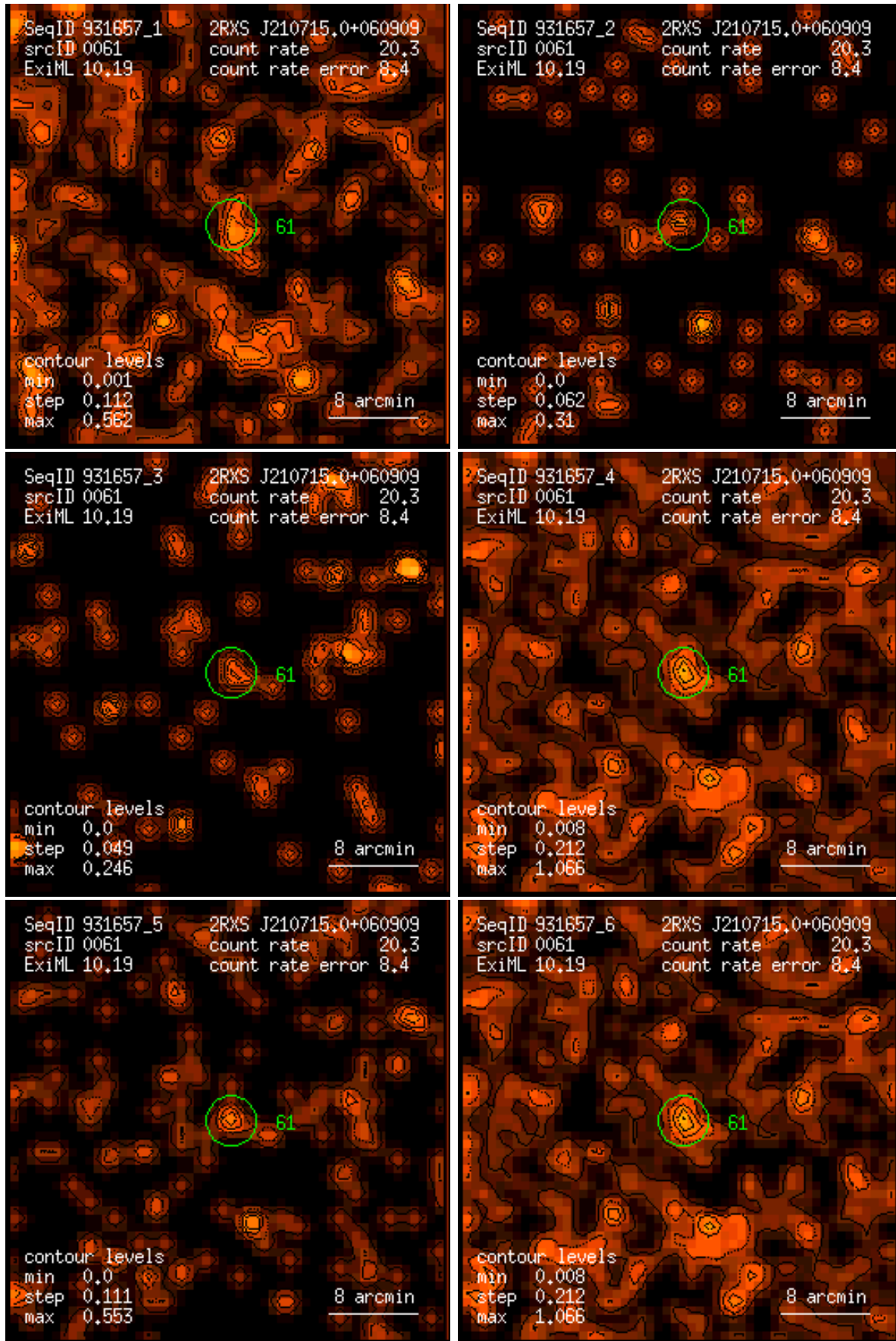
Figure 61: RASS 931657: detection 0061: band rate images, Gaussian filter: (1) PSPC channels 11 – 41, (2) 52 – 90, (3) 91 – 201, (4) 11 – 235, (5) 52 – 201, (6) 11 – 201. Broad band rates in counts/ks. Band rate contour levels in counts/ks/arcmin 2 .
