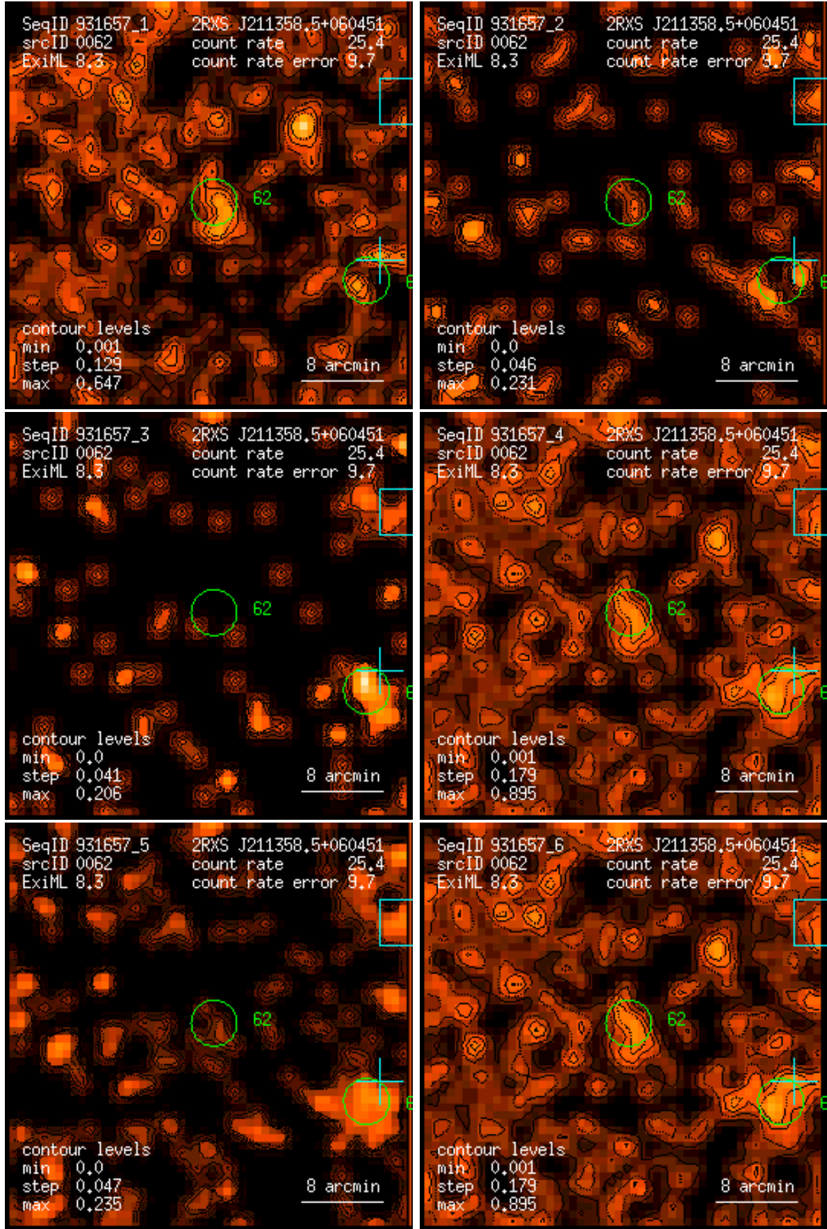
Figure 62: RASS 931657: detection 0062: band rate images, Gaussian filter: (1) PSPC channels 11 – 41, (2) 52 – 90, (3) 91 – 201, (4) 11 – 235, (5) 52 – 201, (6) 11 – 201. Broad band rates in counts/ks. Band rate contour levels in counts/ks/arcmin 2 .
