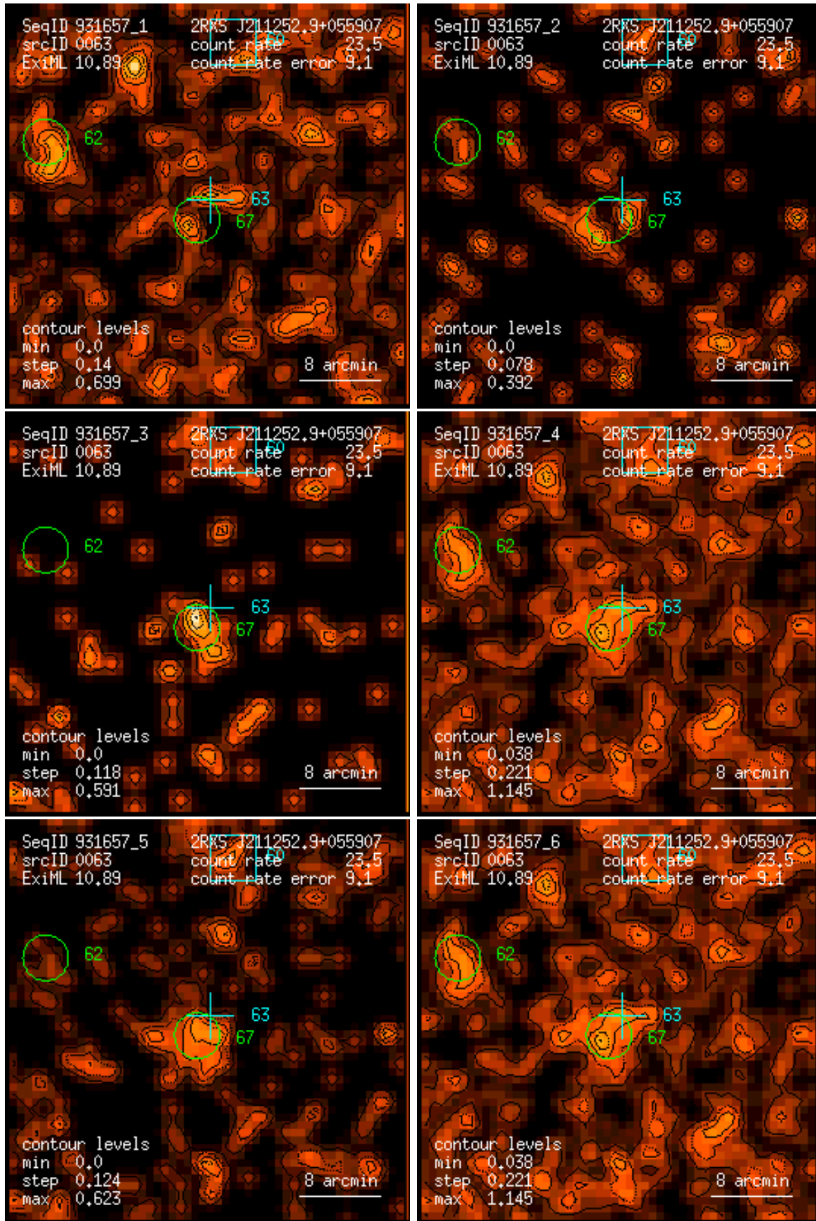
Figure 63: RASS 931657: detection 0063: band rate images, Gaussian filter: (1) PSPC channels 11 – 41, (2) 52 – 90, (3) 91 – 201, (4) 11 – 235, (5) 52 – 201, (6) 11 – 201. Broad band rates in counts/ks. Band rate contour levels in counts/ks/arcmin 2 .
