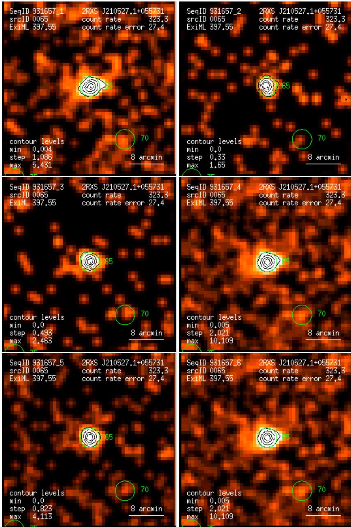
Figure 65: RASS 931657: detection 0065: band rate images, Gaussian filter: (1) PSPC channels 11 – 41, (2) 52 – 90, (3) 91 – 201, (4) 11 – 235, (5) 52 – 201, (6) 11 – 201. Broad band rates in counts/ks. Band rate contour levels in counts/ks/arcmin 2 .
