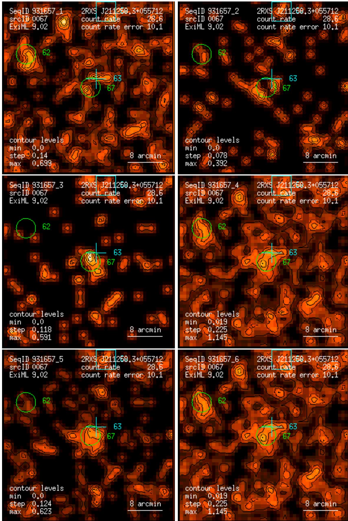
Figure 67: RASS 931657: detection 0067: band rate images, Gaussian filter: (1) PSPC channels 11 – 41, (2) 52 – 90, (3) 91 – 201, (4) 11 – 235, (5) 52 – 201, (6) 11 – 201. Broad band rates in counts/ks. Band rate contour levels in counts/ks/arcmin 2 .
