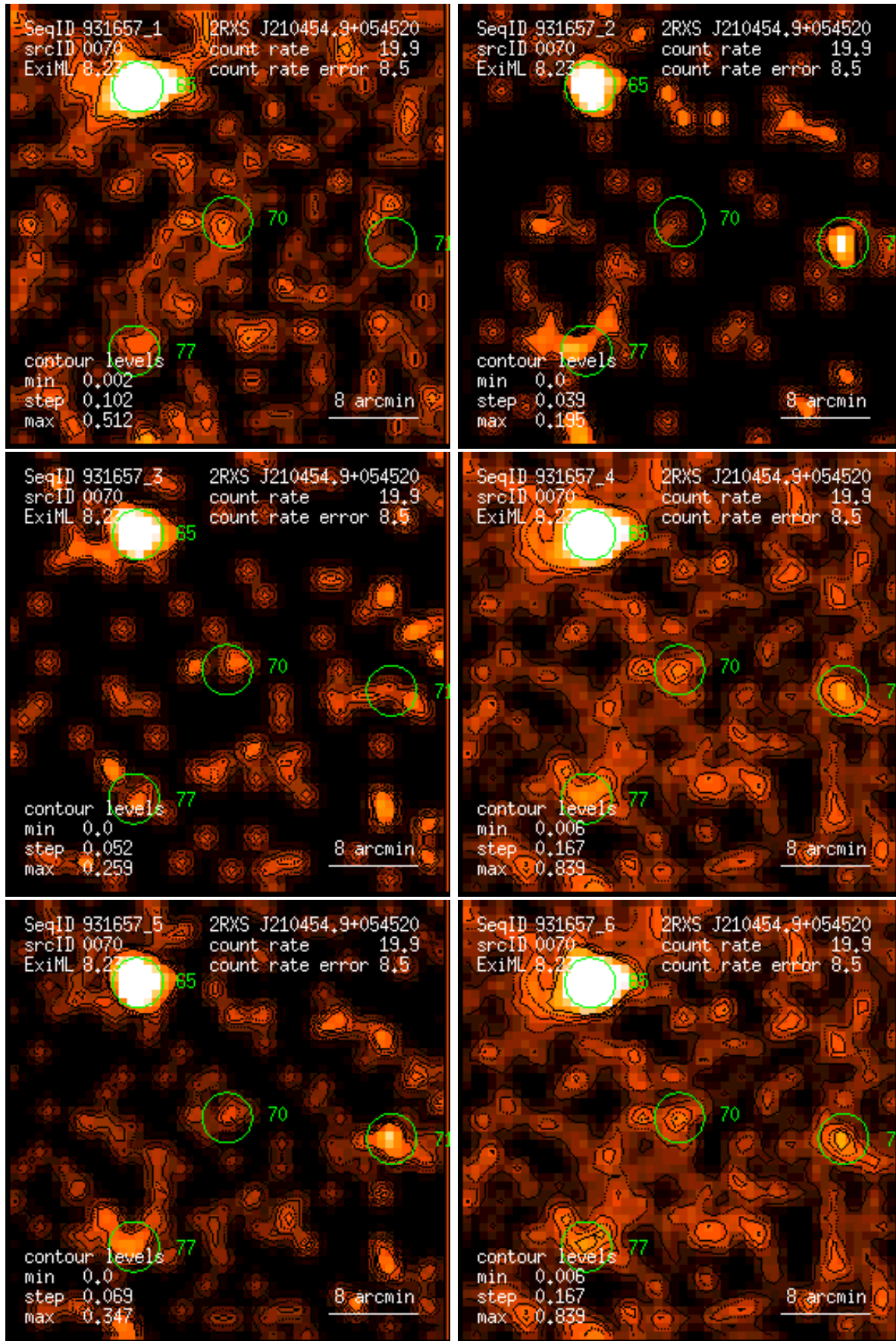
Figure 70: RASS 931657: detection 0070: band rate images, Gaussian filter: (1) PSPC channels 11 – 41, (2) 52 – 90, (3) 91 – 201, (4) 11 – 235, (5) 52 – 201, (6) 11 – 201. Broad band rates in counts/ks. Band rate contour levels in counts/ks/arcmin 2 .
