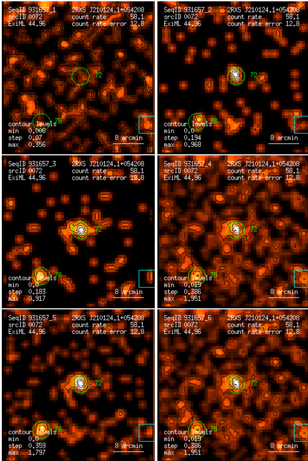
Figure 72: RASS 931657: detection 0072: band rate images, Gaussian filter: (1) PSPC channels 11 – 41, (2) 52 – 90, (3) 91 – 201, (4) 11 – 235, (5) 52 – 201, (6) 11 – 201. Broad band rates in counts/ks. Band rate contour levels in counts/ks/arcmin 2 .
