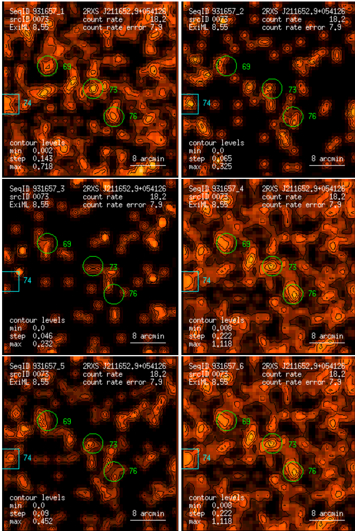
Figure 73: RASS 931657: detection 0073: band rate images, Gaussian filter: (1) PSPC channels 11 – 41, (2) 52 – 90, (3) 91 – 201, (4) 11 – 235, (5) 52 – 201, (6) 11 – 201. Broad band rates in counts/ks. Band rate contour levels in counts/ks/arcmin 2 .
