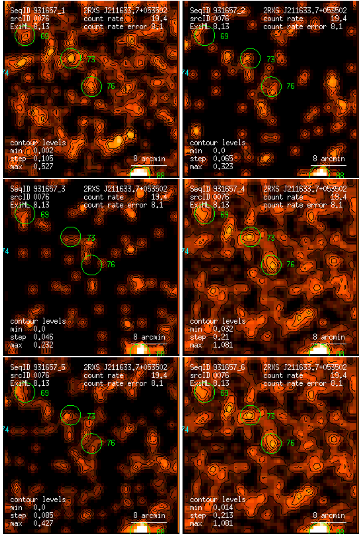
Figure 76: RASS 931657: detection 0076: band rate images, Gaussian filter: (1) PSPC channels 11 – 41, (2) 52 – 90, (3) 91 – 201, (4) 11 – 235, (5) 52 – 201, (6) 11 – 201. Broad band rates in counts/ks. Band rate contour levels in counts/ks/arcmin 2 .
