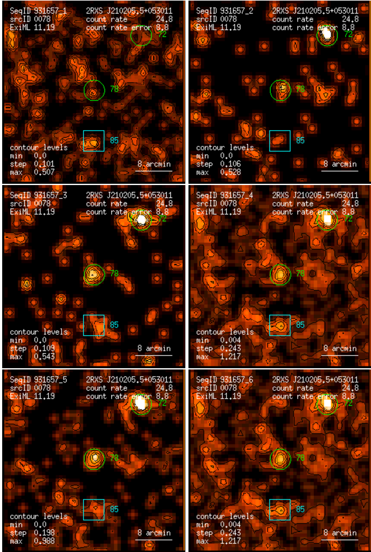
Figure 78: RASS 931657: detection 0078: band rate images, Gaussian filter: (1) PSPC channels 11 – 41, (2) 52 – 90, (3) 91 – 201, (4) 11 – 235, (5) 52 – 201, (6) 11 – 201. Broad band rates in counts/ks. Band rate contour levels in counts/ks/arcmin 2 .
