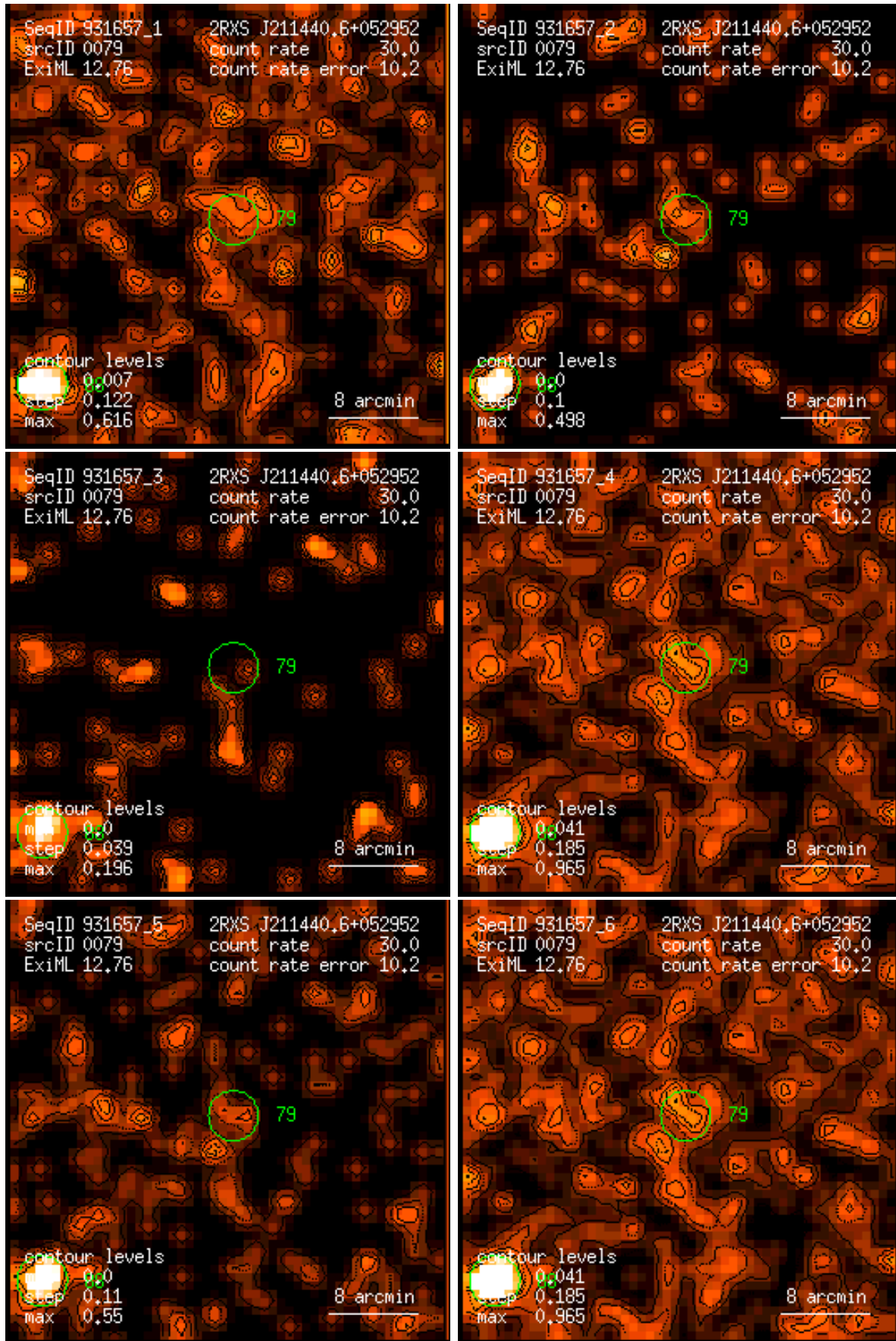
Figure 79: RASS 931657: detection 0079: band rate images, Gaussian filter: (1) PSPC channels 11 – 41, (2) 52 – 90, (3) 91 – 201, (4) 11 – 235, (5) 52 – 201, (6) 11 – 201. Broad band rates in counts/ks. Band rate contour levels in counts/ks/arcmin 2 .
