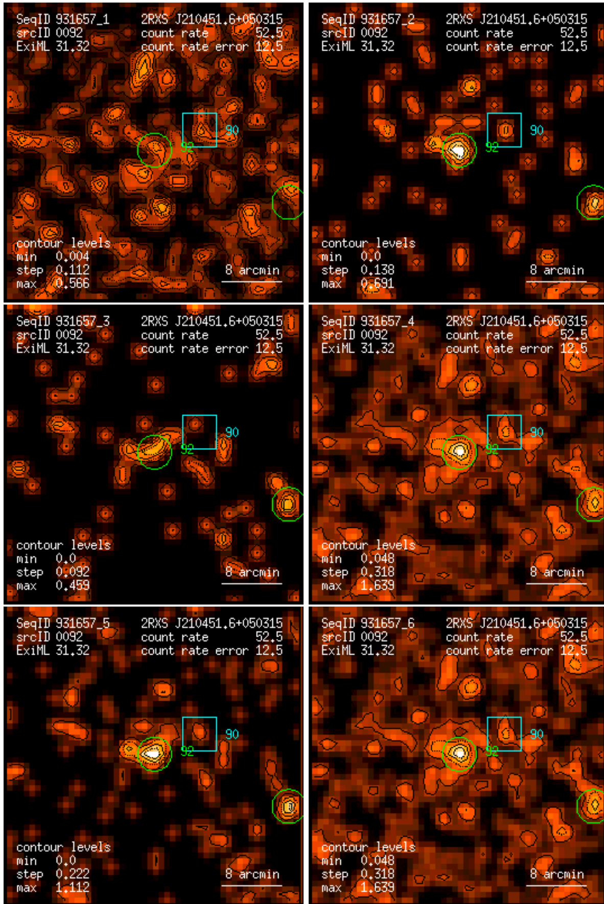
Figure 92: RASS 931657: detection 0092: band rate images, Gaussian filter: (1) PSPC channels 11 – 41, (2) 52 – 90, (3) 91 – 201, (4) 11 – 235, (5) 52 – 201, (6) 11 – 201. Broad band rates in counts/ks. Band rate contour levels in counts/ks/arcmin 2 .
