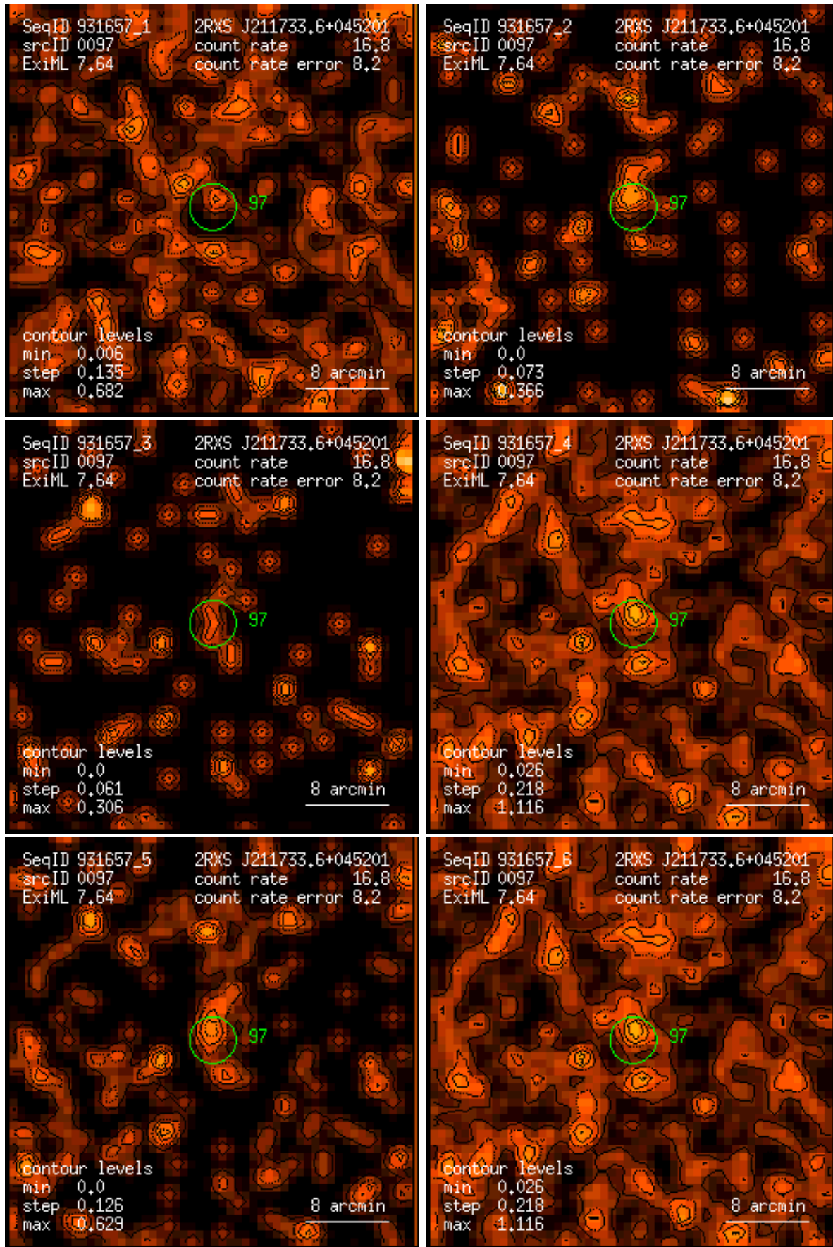
Figure 97: RASS 931657: detection 0097: band rate images, Gaussian filter: (1) PSPC channels 11 – 41, (2) 52 – 90, (3) 91 – 201, (4) 11 – 235, (5) 52 – 201, (6) 11 – 201. Broad band rates in counts/ks. Band rate contour levels in counts/ks/arcmin 2 .
