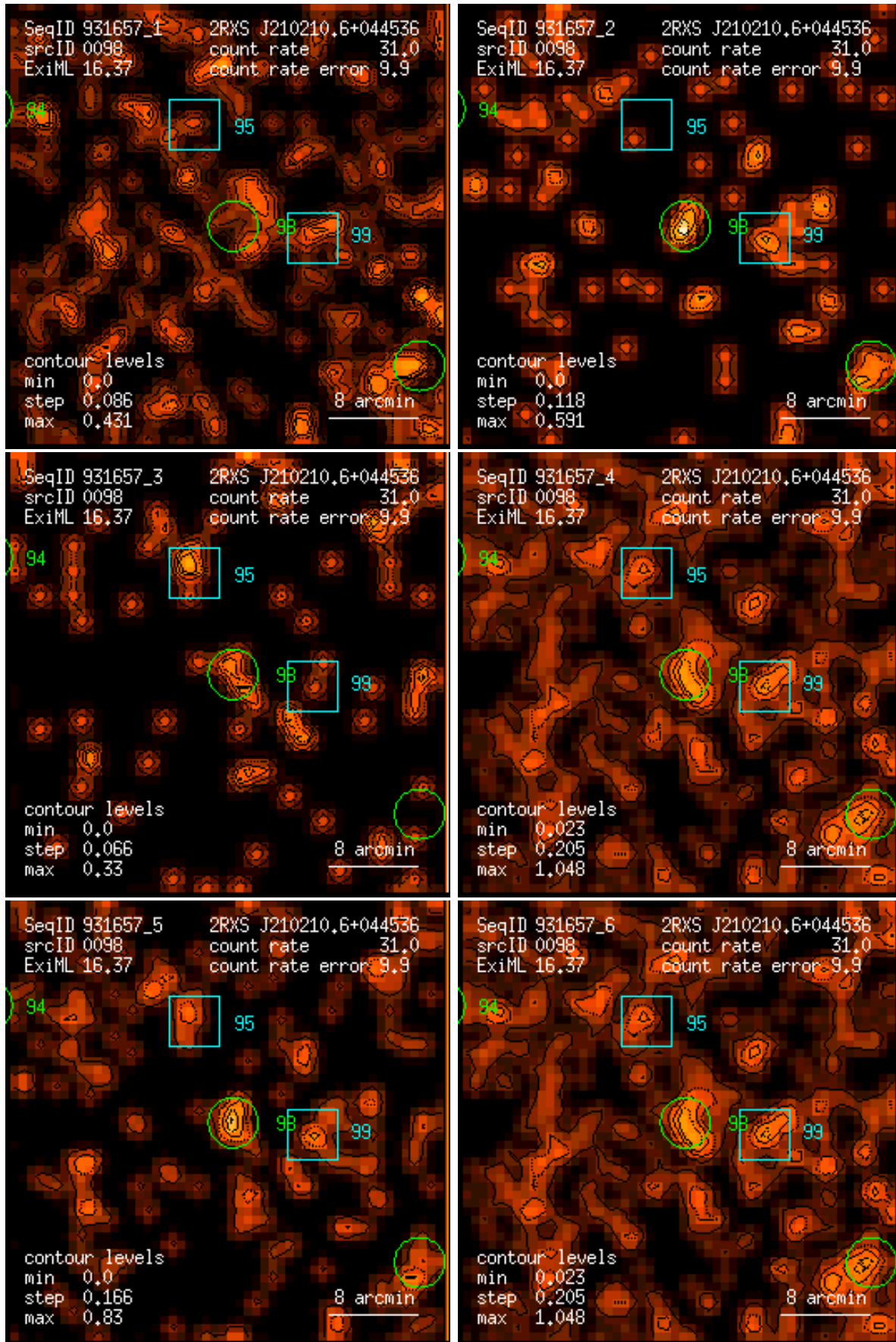
Figure 98: RASS 931657: detection 0098: band rate images, Gaussian filter: (1) PSPC channels 11 – 41, (2) 52 – 90, (3) 91 – 201, (4) 11 – 235, (5) 52 – 201, (6) 11 – 201. Broad band rates in counts/ks. Band rate contour levels in counts/ks/arcmin 2 .
