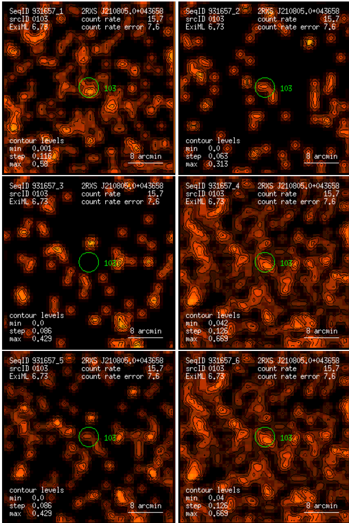
Figure 103: RASS 931657: detection 0103: band rate images, Gaussian filter: (1) PSPC channels 11 – 41, (2) 52 – 90, (3) 91 – 201, (4) 11 – 235, (5) 52 – 201, (6) 11 – 201. Broad band rates in counts/ks. Band rate contour levels in counts/ks/arcmin 2 .
