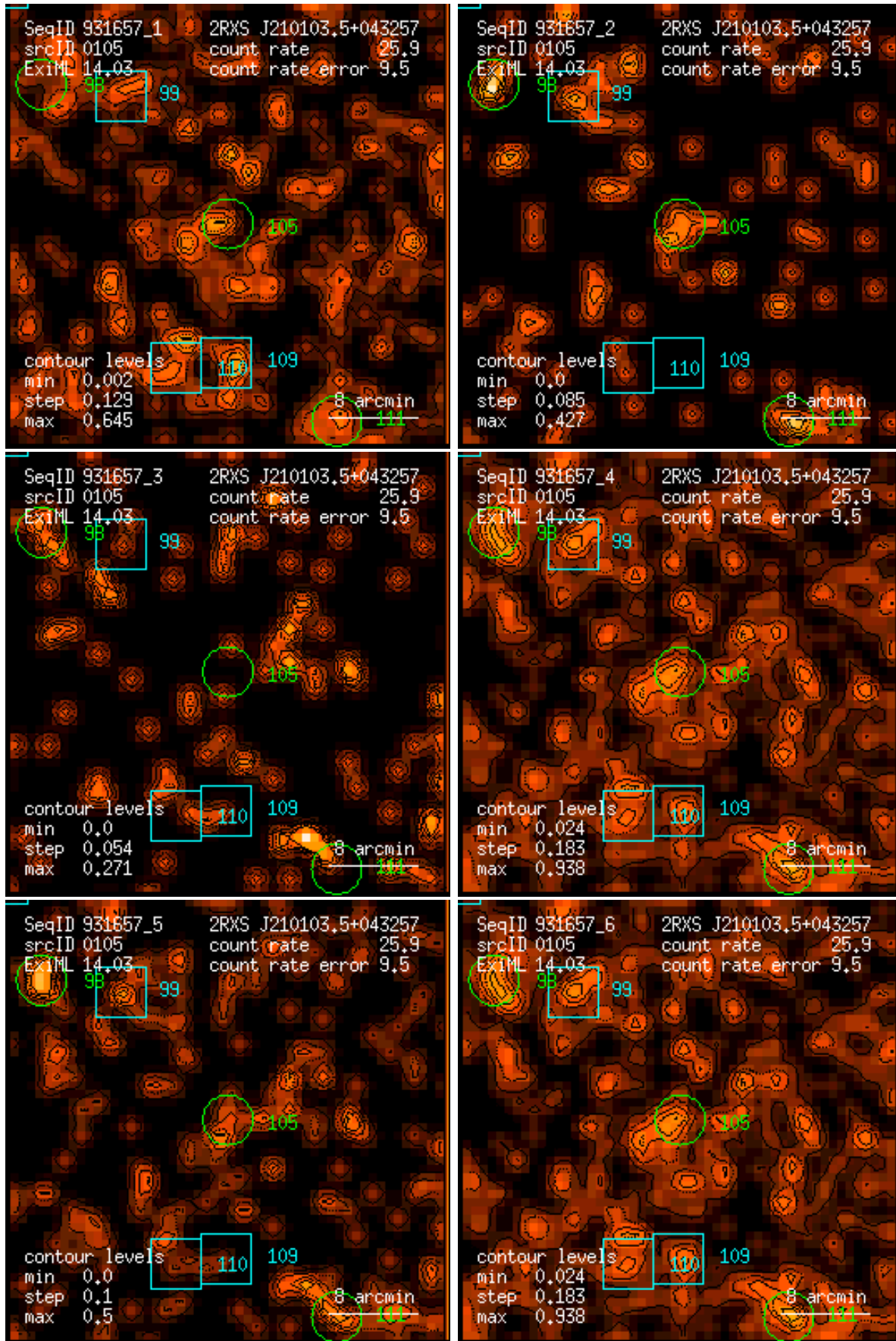
Figure 105: RASS 931657: detection 0105: band rate images, Gaussian filter: (1) PSPC channels 11 – 41, (2) 52 – 90, (3) 91 – 201, (4) 11 – 235, (5) 52 – 201, (6) 11 – 201. Broad band rates in counts/ks. Band rate contour levels in counts/ks/arcmin 2 .
