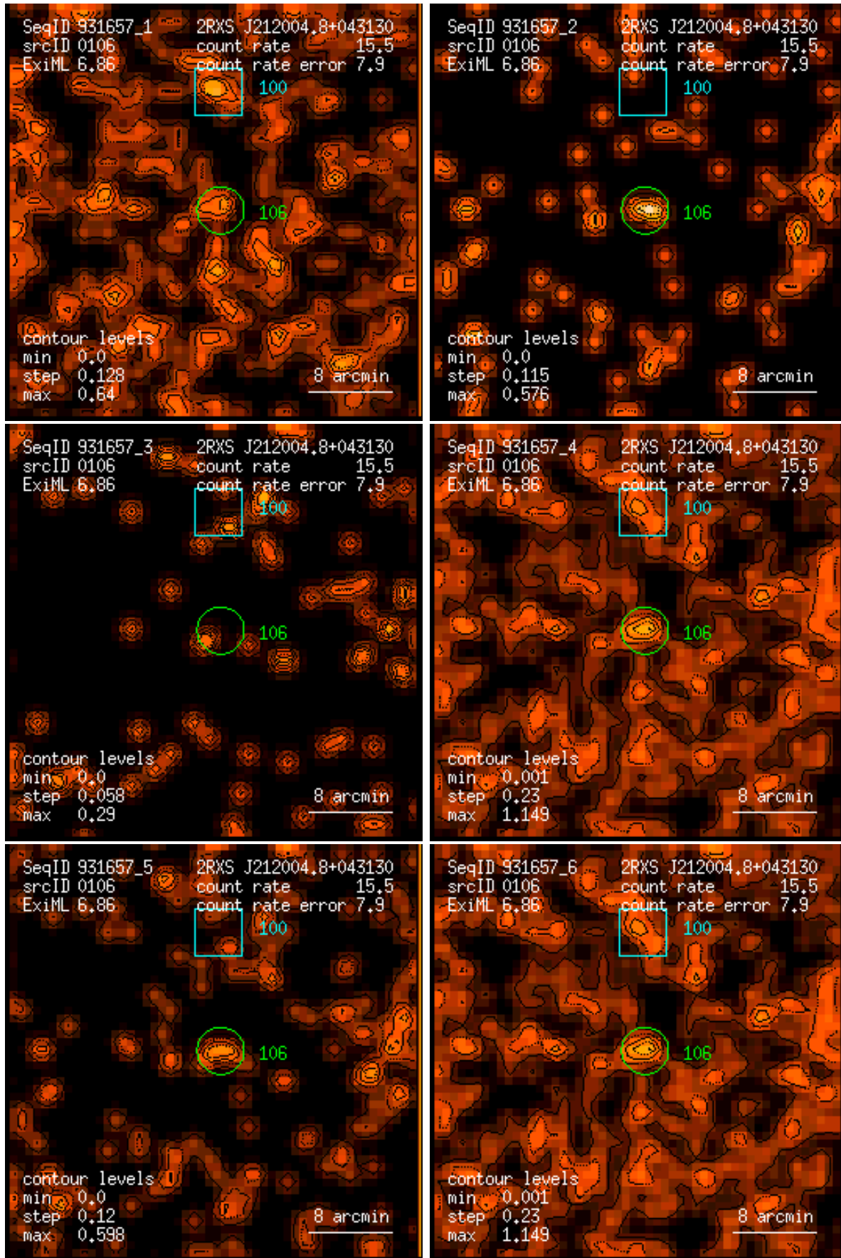
Figure 106: RASS 931657: detection 0106: band rate images, Gaussian filter: (1) PSPC channels 11 – 41, (2) 52 – 90, (3) 91 – 201, (4) 11 – 235, (5) 52 – 201, (6) 11 – 201. Broad band rates in counts/ks. Band rate contour levels in counts/ks/arcmin 2 .
