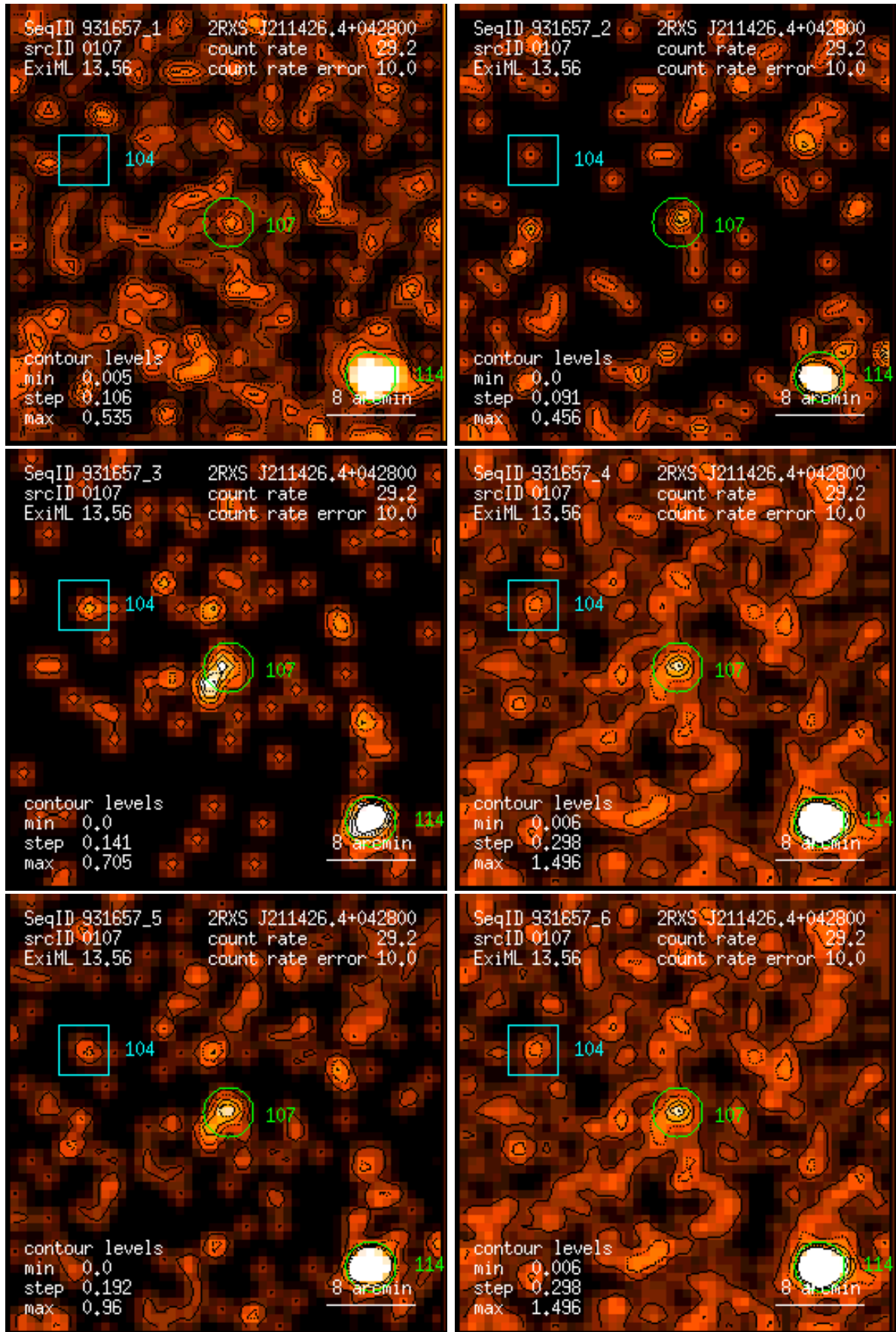
Figure 107: RASS 931657: detection 0107: band rate images, Gaussian filter: (1) PSPC channels 11 – 41, (2) 52 – 90, (3) 91 – 201, (4) 11 – 235, (5) 52 – 201, (6) 11 – 201. Broad band rates in counts/ks. Band rate contour levels in counts/ks/arcmin 2 .
