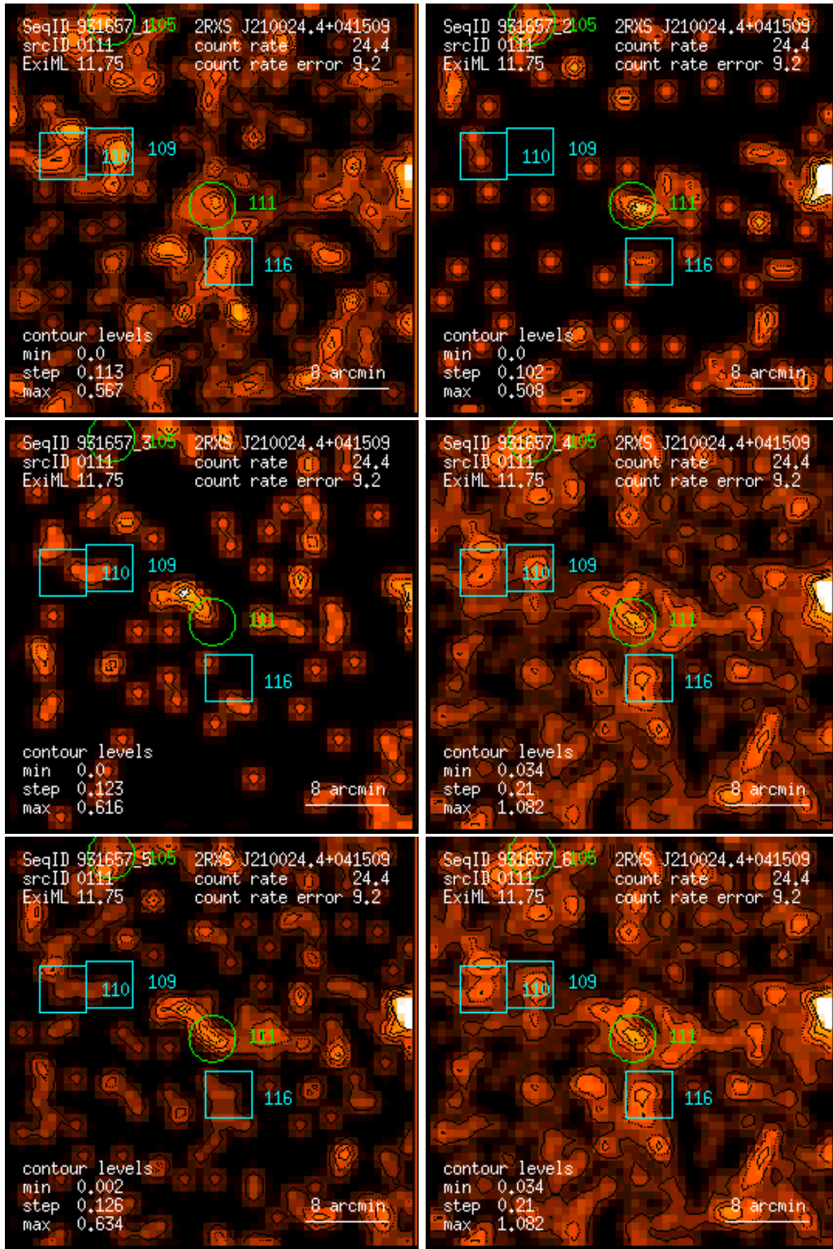
Figure 111: RASS 931657: detection 0111: band rate images, Gaussian filter: (1) PSPC channels 11 – 41, (2) 52 – 90, (3) 91 – 201, (4) 11 – 235, (5) 52 – 201, (6) 11 – 201. Broad band rates in counts/ks. Band rate contour levels in counts/ks/arcmin 2 .
