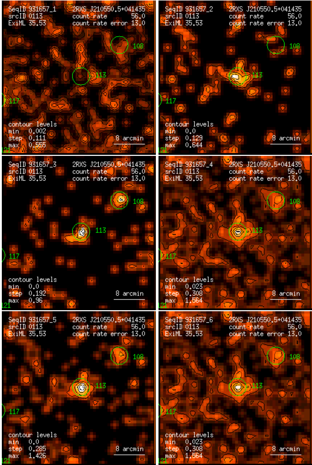
Figure 113: RASS 931657: detection 0113: band rate images, Gaussian filter: (1) PSPC channels 11 – 41, (2) 52 – 90, (3) 91 – 201, (4) 11 – 235, (5) 52 – 201, (6) 11 – 201. Broad band rates in counts/ks. Band rate contour levels in counts/ks/arcmin 2 .
