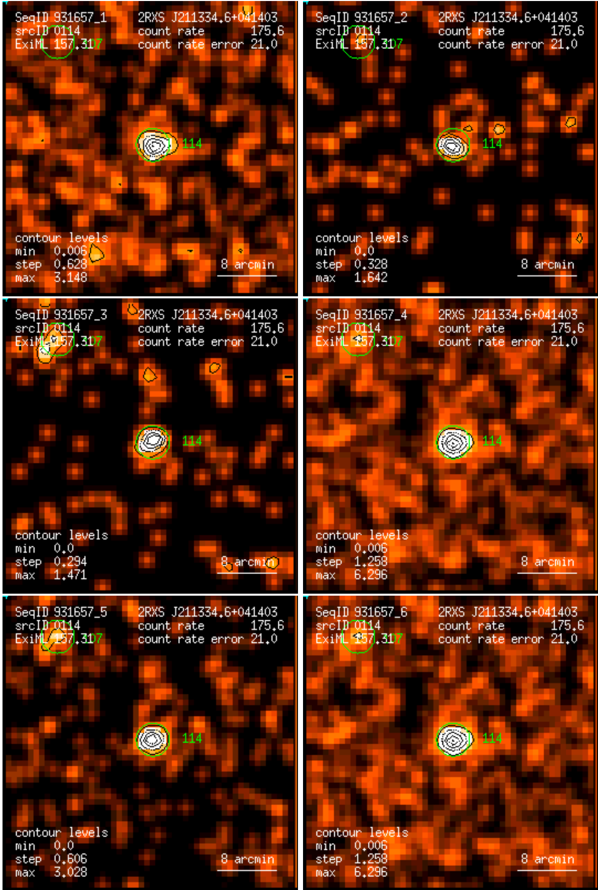
Figure 114: RASS 931657: detection 0114: band rate images, Gaussian filter: (1) PSPC channels 11 – 41, (2) 52 – 90, (3) 91 – 201, (4) 11 – 235, (5) 52 – 201, (6) 11 – 201. Broad band rates in counts/ks. Band rate contour levels in counts/ks/arcmin 2 .
