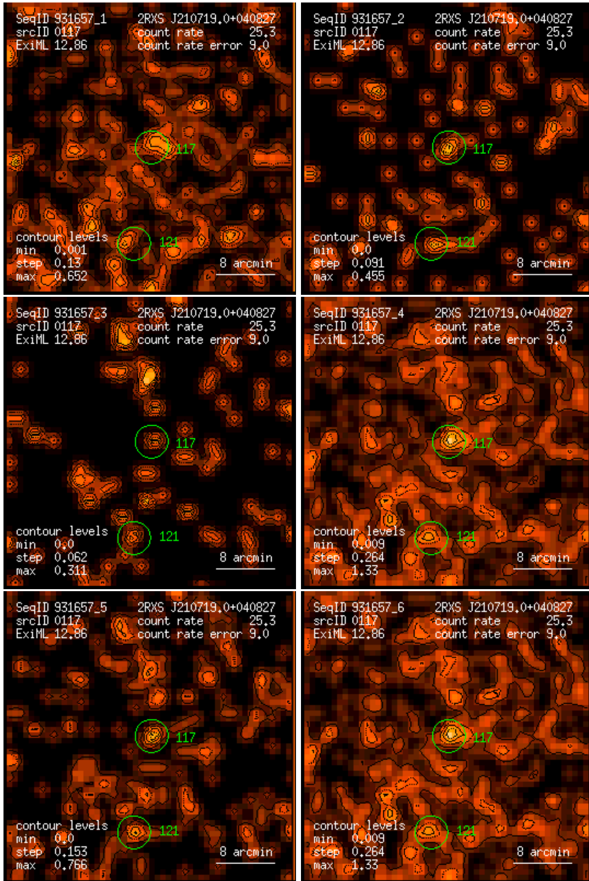
Figure 117: RASS 931657: detection 0117: band rate images, Gaussian filter: (1) PSPC channels 11 – 41, (2) 52 – 90, (3) 91 – 201, (4) 11 – 235, (5) 52 – 201, (6) 11 – 201. Broad band rates in counts/ks. Band rate contour levels in counts/ks/arcmin 2 .
