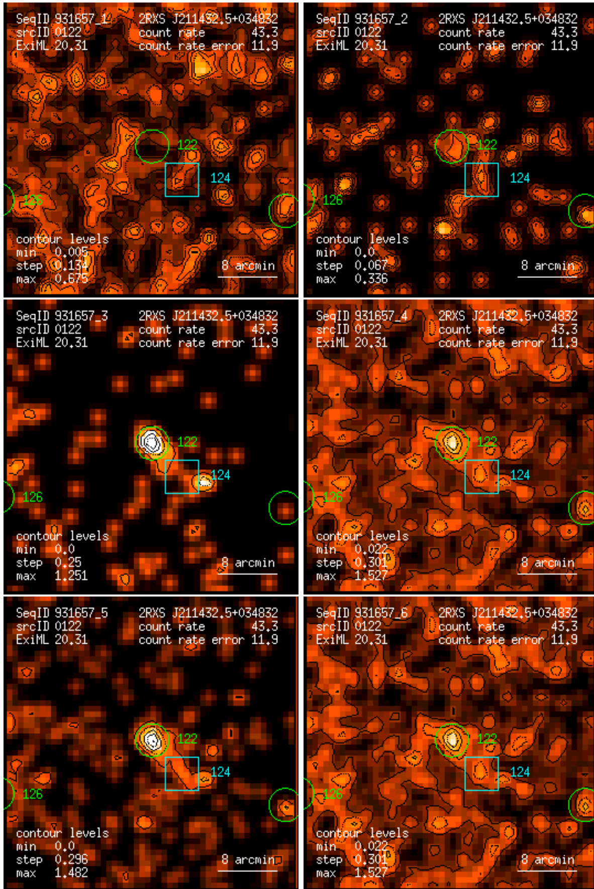
Figure 122: RASS 931657: detection 0122: band rate images, Gaussian filter: (1) PSPC channels 11 – 41, (2) 52 – 90, (3) 91 – 201, (4) 11 – 235, (5) 52 – 201, (6) 11 – 201. Broad band rates in counts/ks. Band rate contour levels in counts/ks/arcmin 2 .
