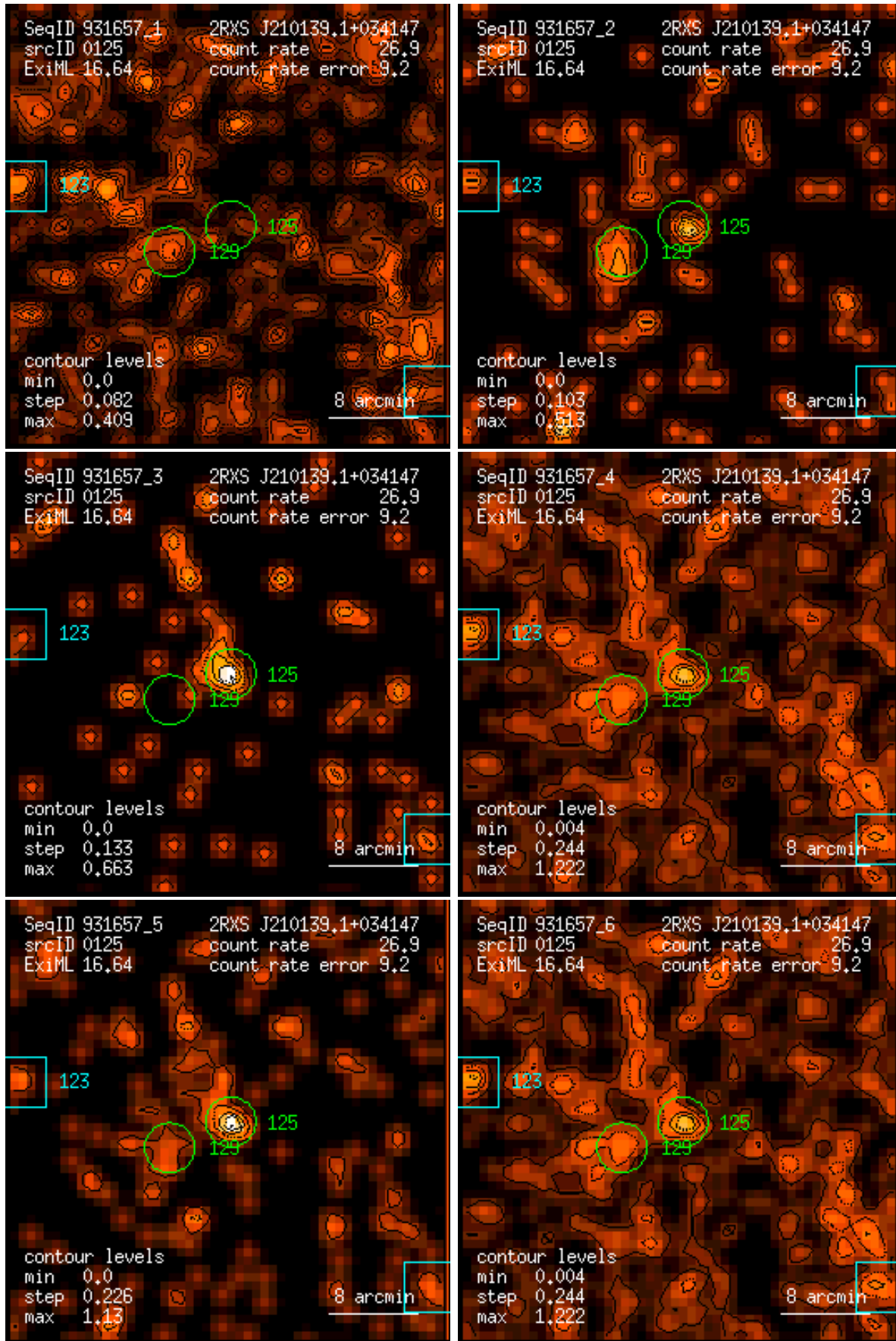
Figure 125: RASS 931657: detection 0125: band rate images, Gaussian filter: (1) PSPC channels 11 – 41, (2) 52 – 90, (3) 91 – 201, (4) 11 – 235, (5) 52 – 201, (6) 11 – 201. Broad band rates in counts/ks. Band rate contour levels in counts/ks/arcmin 2 .
