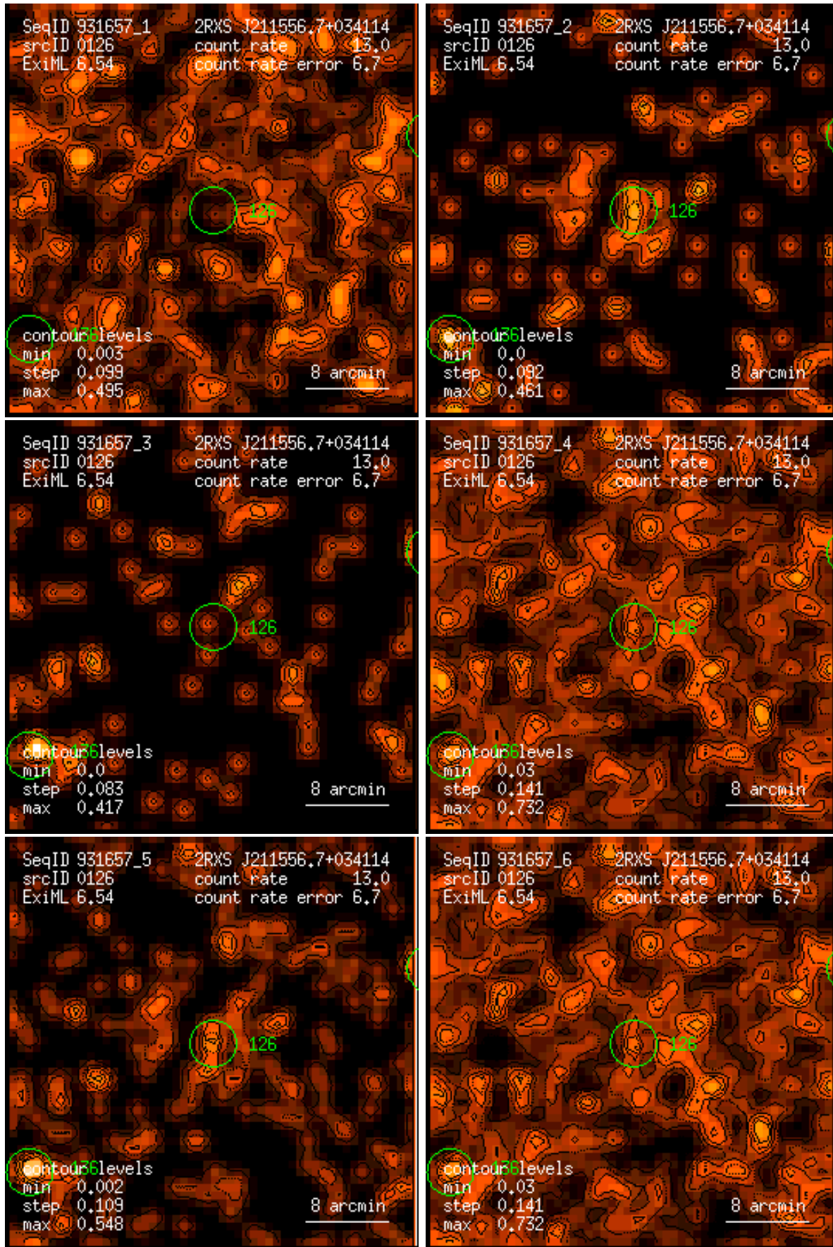
Figure 126: RASS 931657: detection 0126: band rate images, Gaussian filter: (1) PSPC channels 11 – 41, (2) 52 – 90, (3) 91 – 201, (4) 11 – 235, (5) 52 – 201, (6) 11 – 201. Broad band rates in counts/ks. Band rate contour levels in counts/ks/arcmin 2 .
