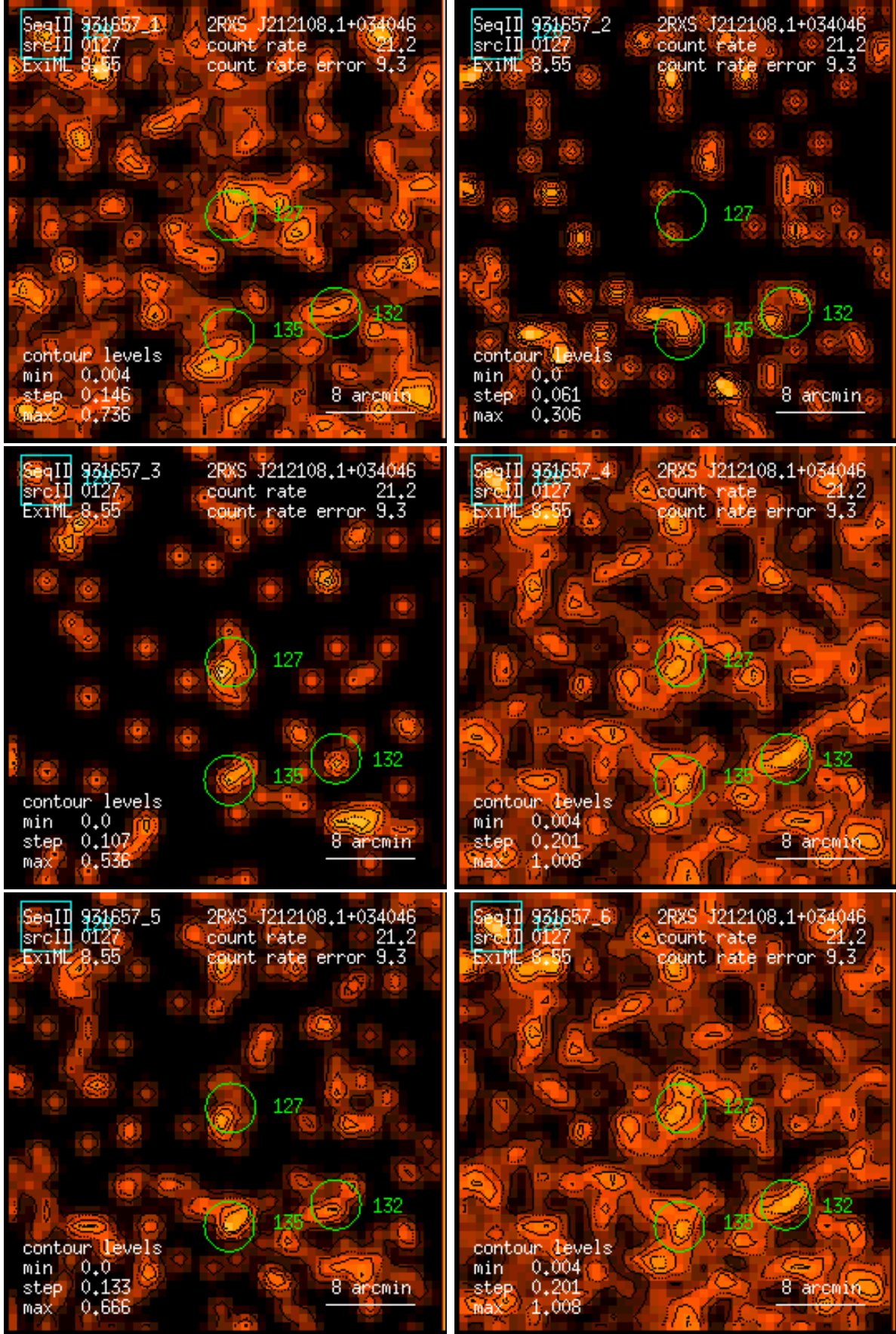
Figure 127: RASS 931657: detection 0127: band rate images, Gaussian filter: (1) PSPC channels 11 – 41, (2) 52 – 90, (3) 91 – 201, (4) 11 – 235, (5) 52 – 201, (6) 11 – 201. Broad band rates in counts/ks. Band rate contour levels in counts/ks/arcmin 2 .
