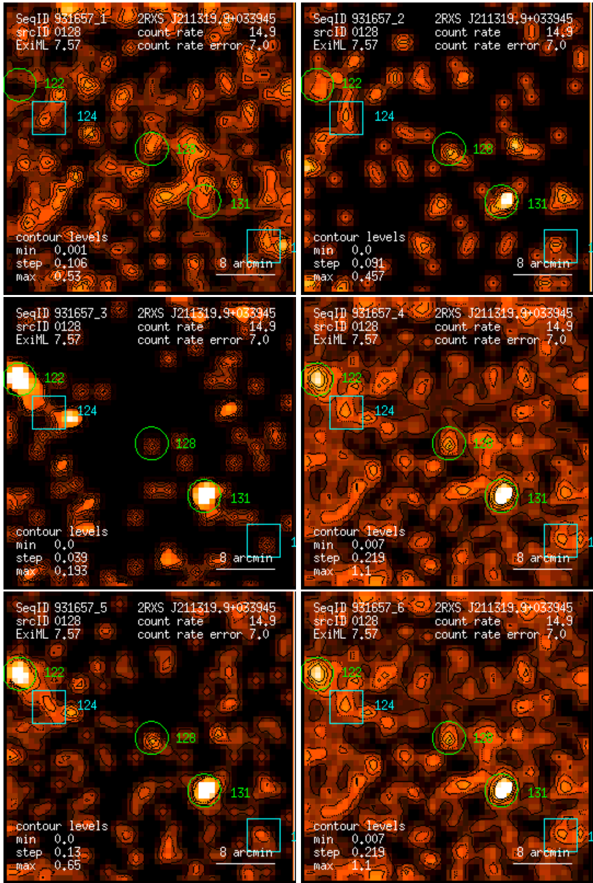
Figure 128: RASS 931657: detection 0128: band rate images, Gaussian filter: (1) PSPC channels 11 – 41, (2) 52 – 90, (3) 91 – 201, (4) 11 – 235, (5) 52 – 201, (6) 11 – 201. Broad band rates in counts/ks. Band rate contour levels in counts/ks/arcmin 2 .
