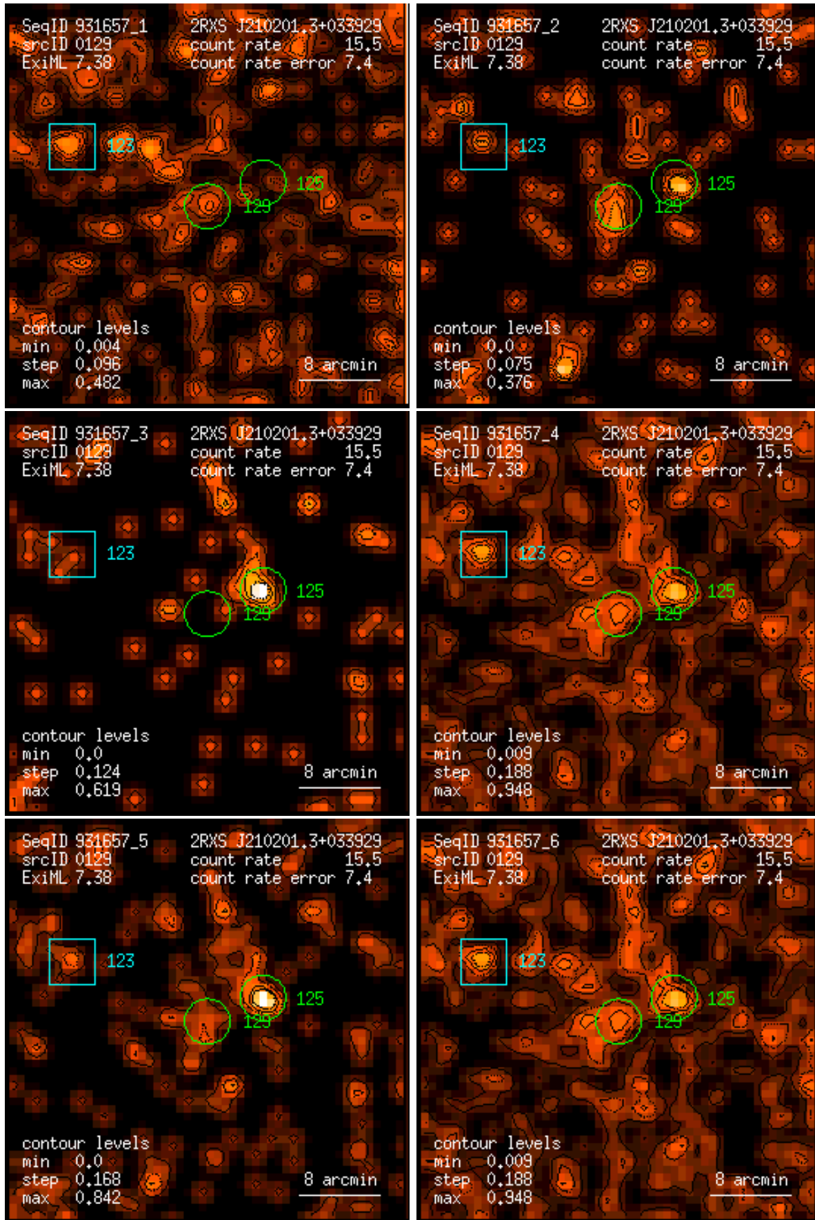
Figure 129: RASS 931657: detection 0129: band rate images, Gaussian filter: (1) PSPC channels 11 – 41, (2) 52 – 90, (3) 91 – 201, (4) 11 – 235, (5) 52 – 201, (6) 11 – 201. Broad band rates in counts/ks. Band rate contour levels in counts/ks/arcmin 2 .
