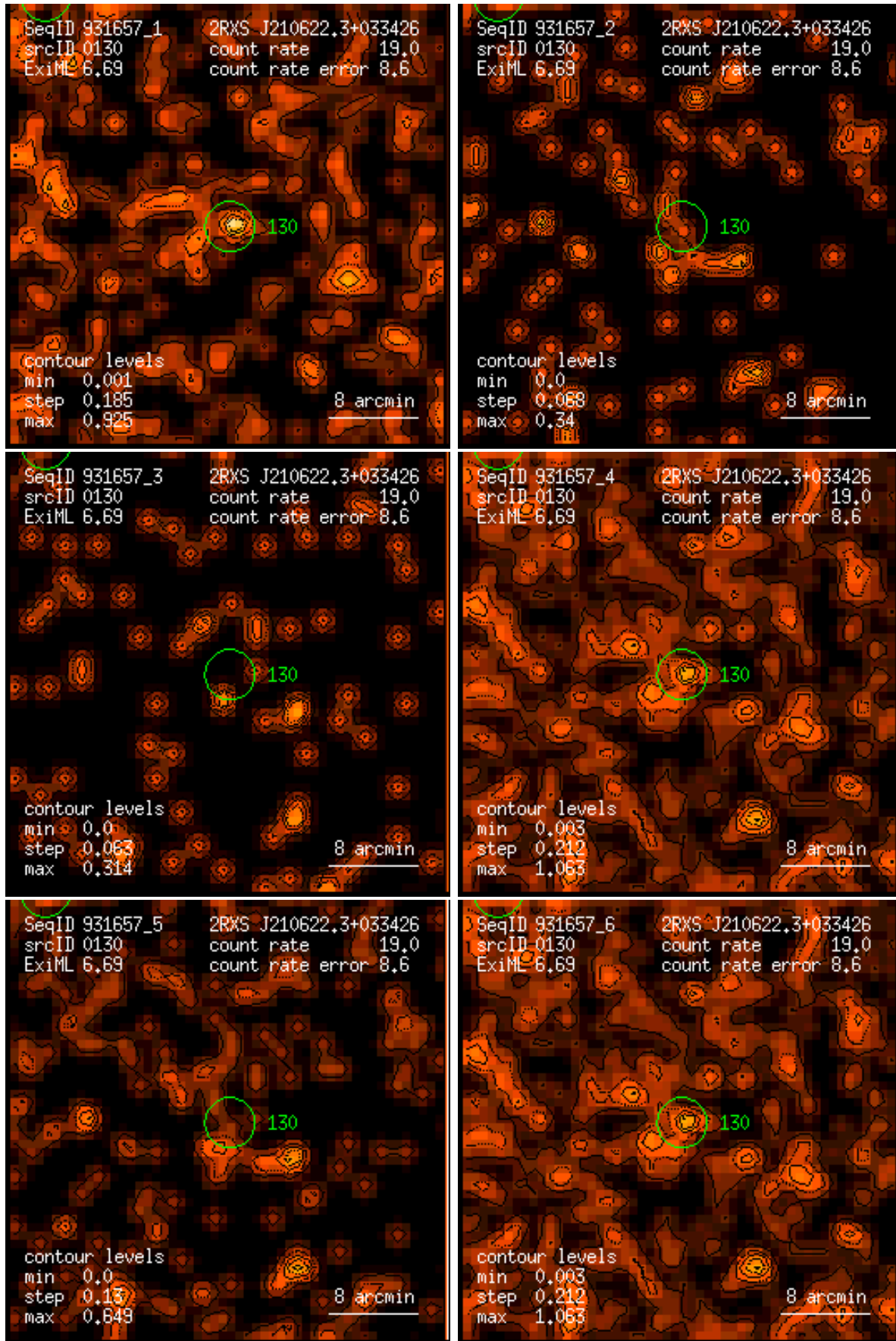
Figure 130: RASS 931657: detection 0130: band rate images, Gaussian filter: (1) PSPC channels 11 – 41, (2) 52 – 90, (3) 91 – 201, (4) 11 – 235, (5) 52 – 201, (6) 11 – 201. Broad band rates in counts/ks. Band rate contour levels in counts/ks/arcmin 2 .
