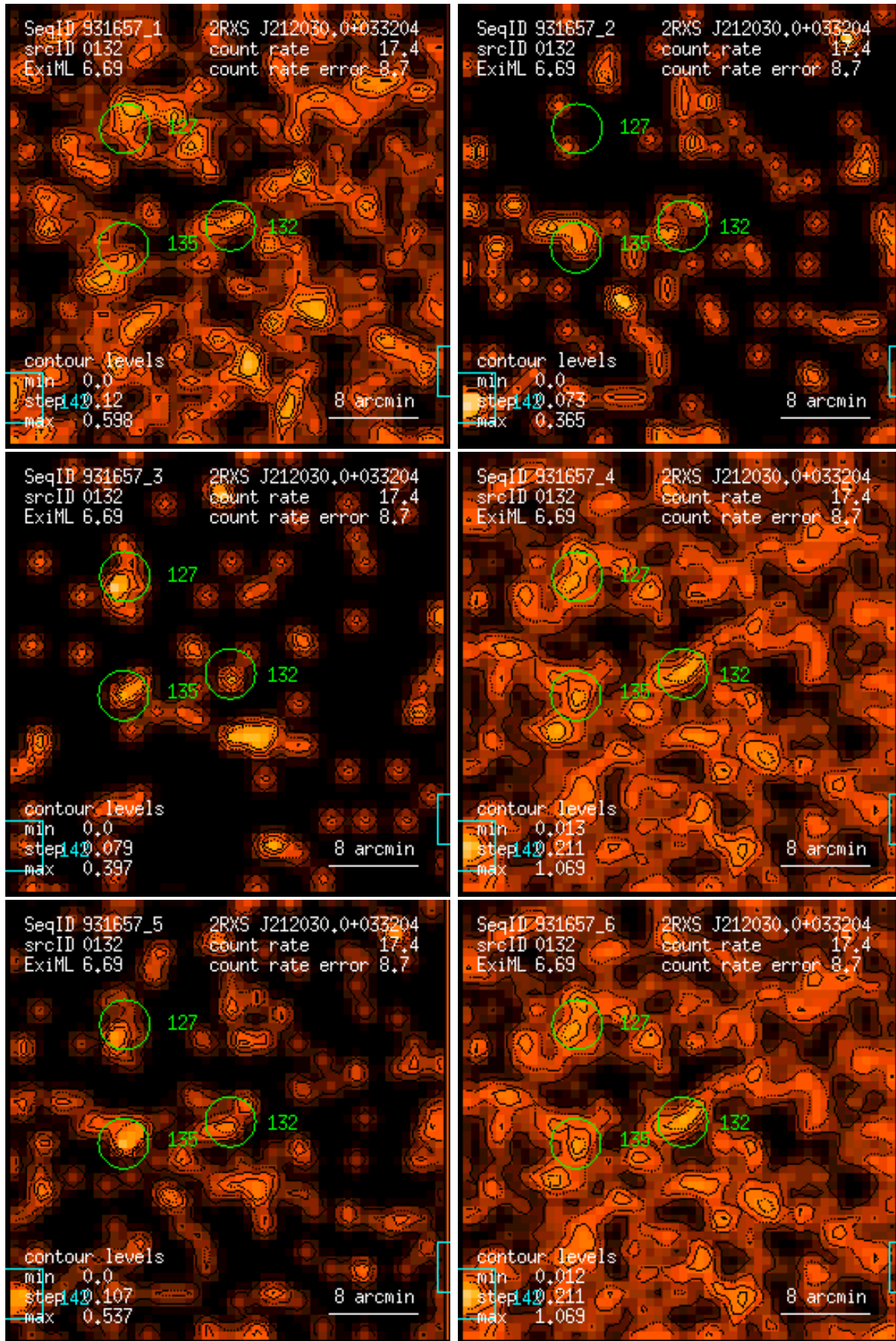
Figure 132: RASS 931657: detection 0132: band rate images, Gaussian filter: (1) PSPC channels 11 – 41, (2) 52 – 90, (3) 91 – 201, (4) 11 – 235, (5) 52 – 201, (6) 11 – 201. Broad band rates in counts/ks. Band rate contour levels in counts/ks/arcmin 2 .
