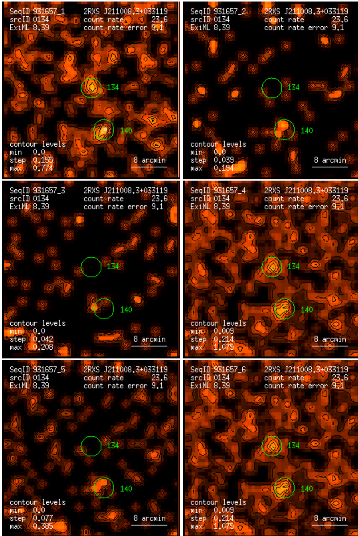
Figure 134: RASS 931657: detection 0134: band rate images, Gaussian filter: (1) PSPC channels 11 – 41, (2) 52 – 90, (3) 91 – 201, (4) 11 – 235, (5) 52 – 201, (6) 11 – 201. Broad band rates in counts/ks. Band rate contour levels in counts/ks/arcmin 2 .
