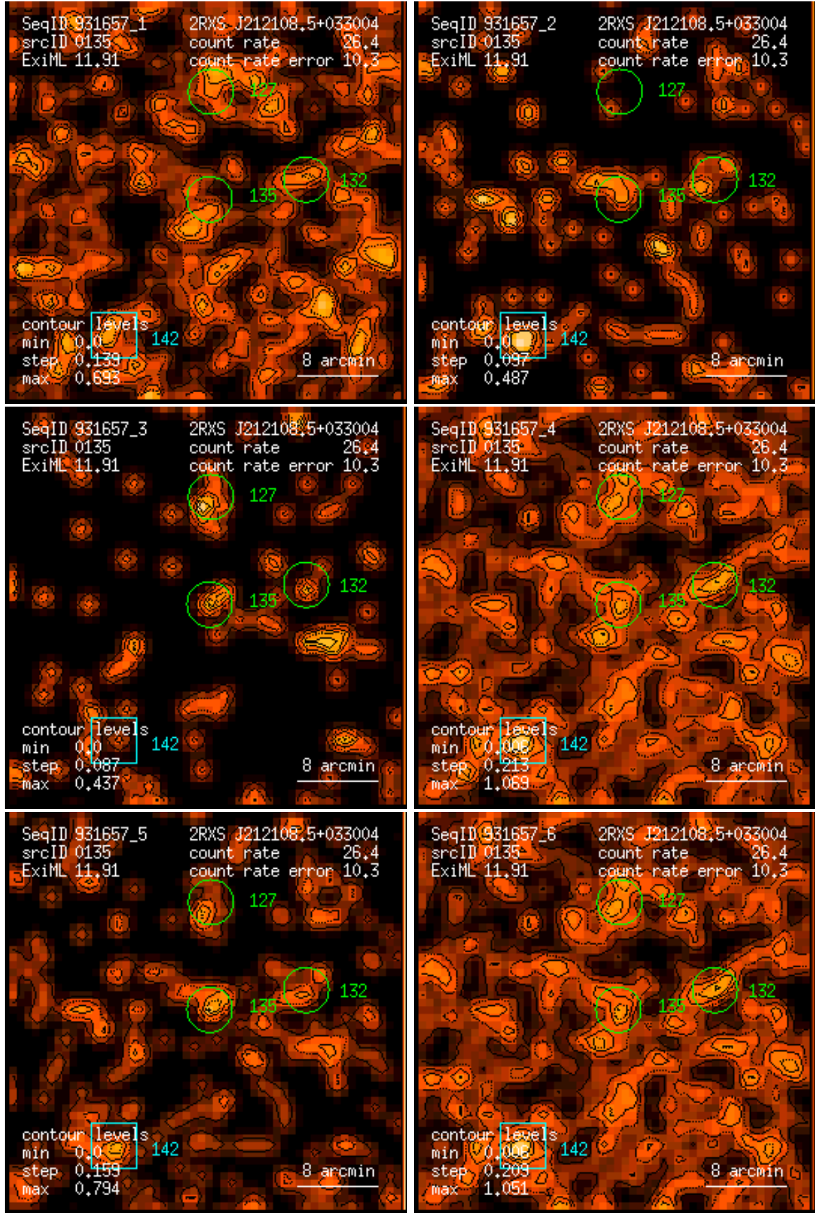
Figure 135: RASS 931657: detection 0135: band rate images, Gaussian filter: (1) PSPC channels 11 – 41, (2) 52 – 90, (3) 91 – 201, (4) 11 – 235, (5) 52 – 201, (6) 11 – 201. Broad band rates in counts/ks. Band rate contour levels in counts/ks/arcmin 2 .
