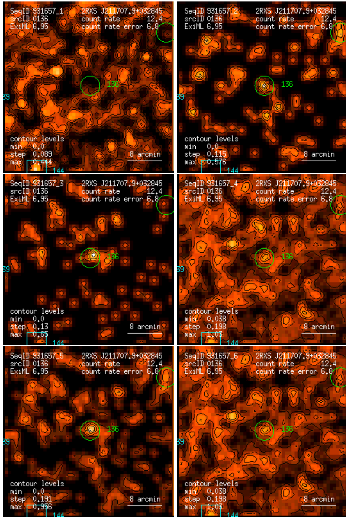
Figure 136: RASS 931657: detection 0136: band rate images, Gaussian filter: (1) PSPC channels 11 – 41, (2) 52 – 90, (3) 91 – 201, (4) 11 – 235, (5) 52 – 201, (6) 11 – 201. Broad band rates in counts/ks. Band rate contour levels in counts/ks/arcmin 2 .
