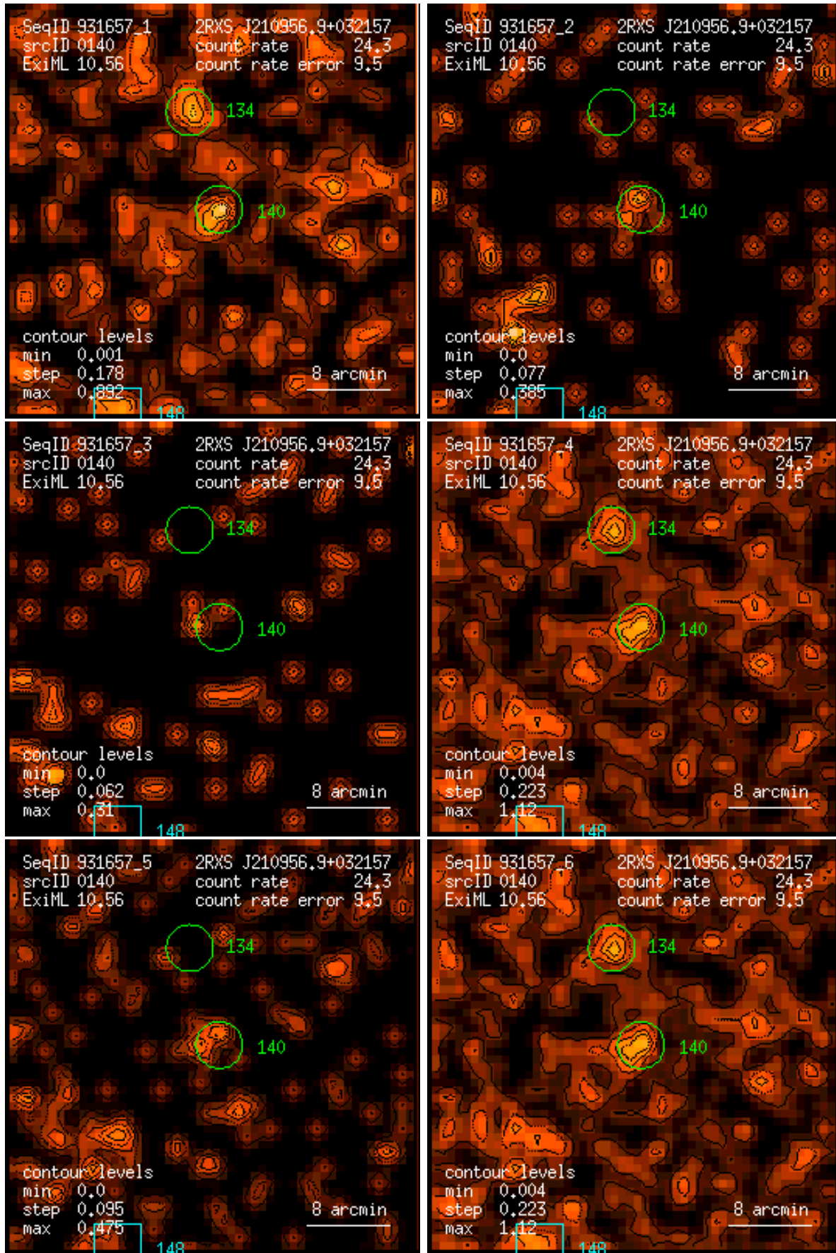
Figure 140: RASS 931657: detection 0140: band rate images, Gaussian filter: (1) PSPC channels 11 – 41, (2) 52 – 90, (3) 91 – 201, (4) 11 – 235, (5) 52 – 201, (6) 11 – 201. Broad band rates in counts/ks. Band rate contour levels in counts/ks/arcmin 2 .
