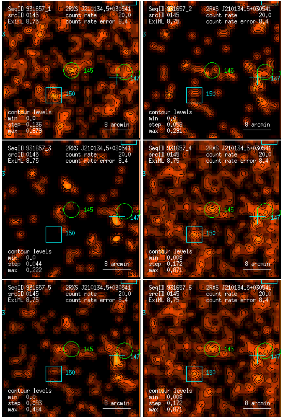
Figure 145: RASS 931657: detection 0145: band rate images, Gaussian filter: (1) PSPC channels 11 – 41, (2) 52 – 90, (3) 91 – 201, (4) 11 – 235, (5) 52 – 201, (6) 11 – 201. Broad band rates in counts/ks. Band rate contour levels in counts/ks/arcmin 2 .
