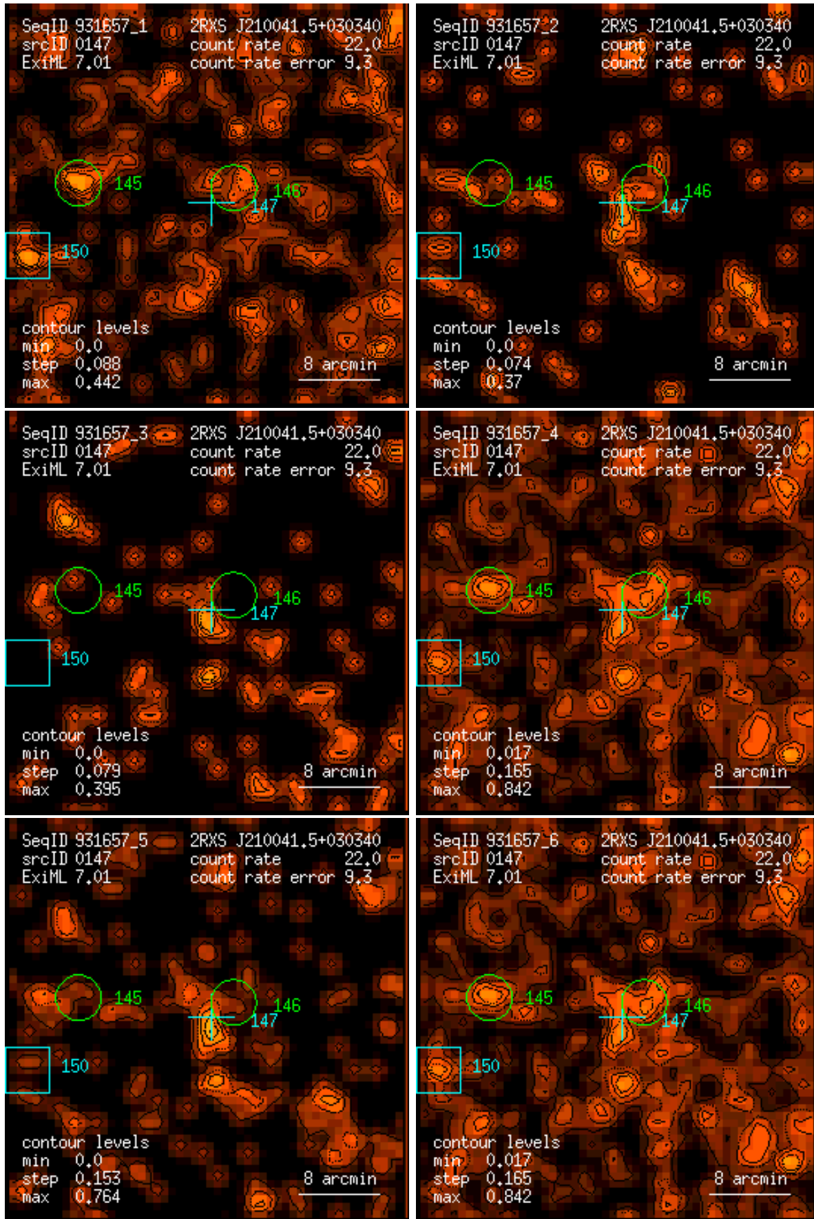
Figure 147: RASS 931657: detection 0147: band rate images, Gaussian filter: (1) PSPC channels 11 – 41, (2) 52 – 90, (3) 91 – 201, (4) 11 – 235, (5) 52 – 201, (6) 11 – 201. Broad band rates in counts/ks. Band rate contour levels in counts/ks/arcmin 2 .
