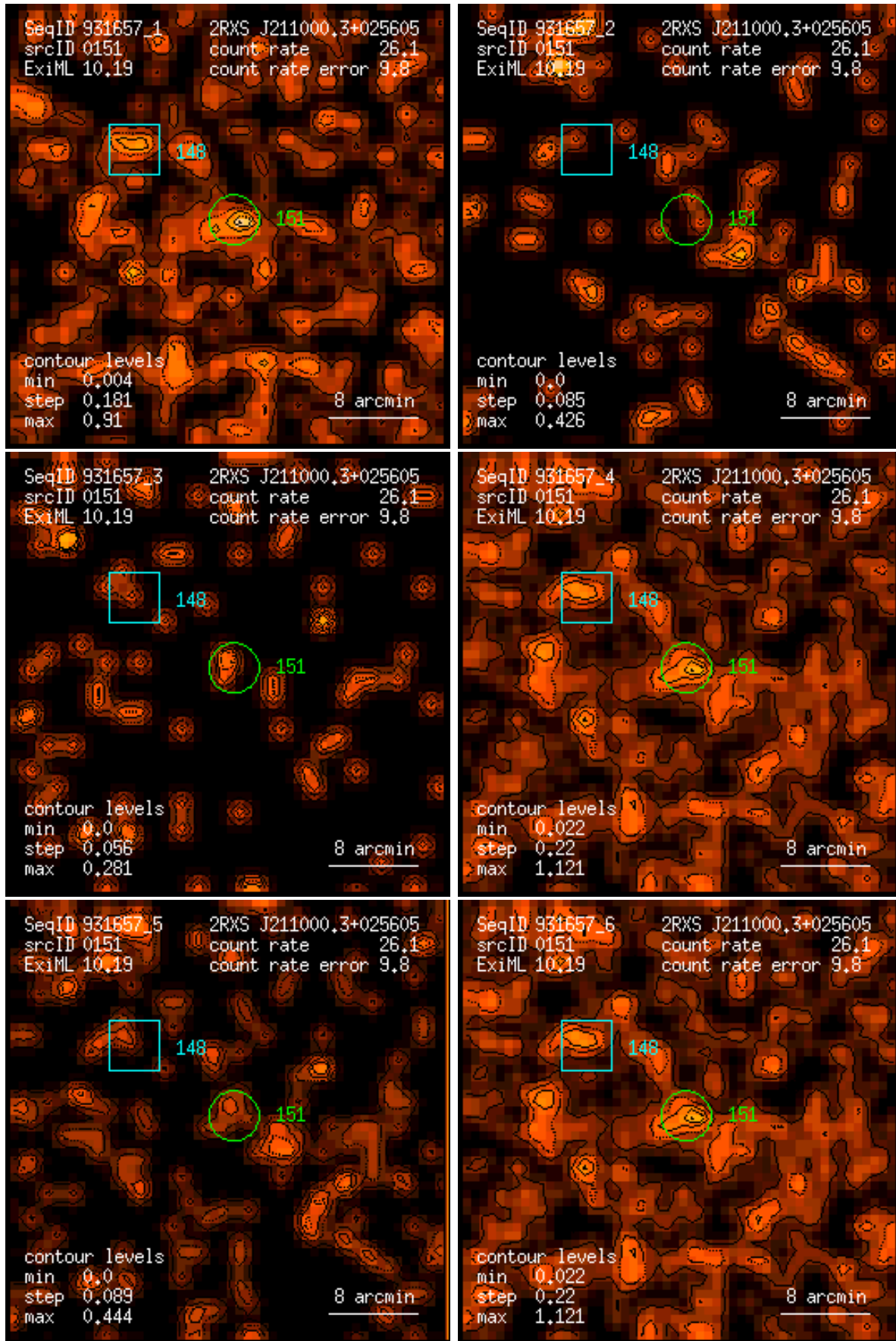
Figure 151: RASS 931657: detection 0151: band rate images, Gaussian filter: (1) PSPC channels 11 – 41, (2) 52 – 90, (3) 91 – 201, (4) 11 – 235, (5) 52 – 201, (6) 11 – 201. Broad band rates in counts/ks. Band rate contour levels in counts/ks/arcmin 2 .
