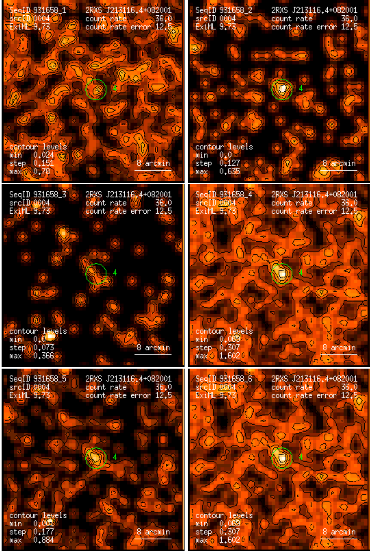
Figure 4: RASS 931658: detection 0004: band rate images, Gaussian filter: (1) PSPC channels 11 – 41, (2) 52 – 90, (3) 91 – 201, (4) 11 – 235, (5) 52 – 201, (6) 11 – 201. Broad band rates in counts/ks. Band rate contour levels in counts/ks/arcmin 2 .
