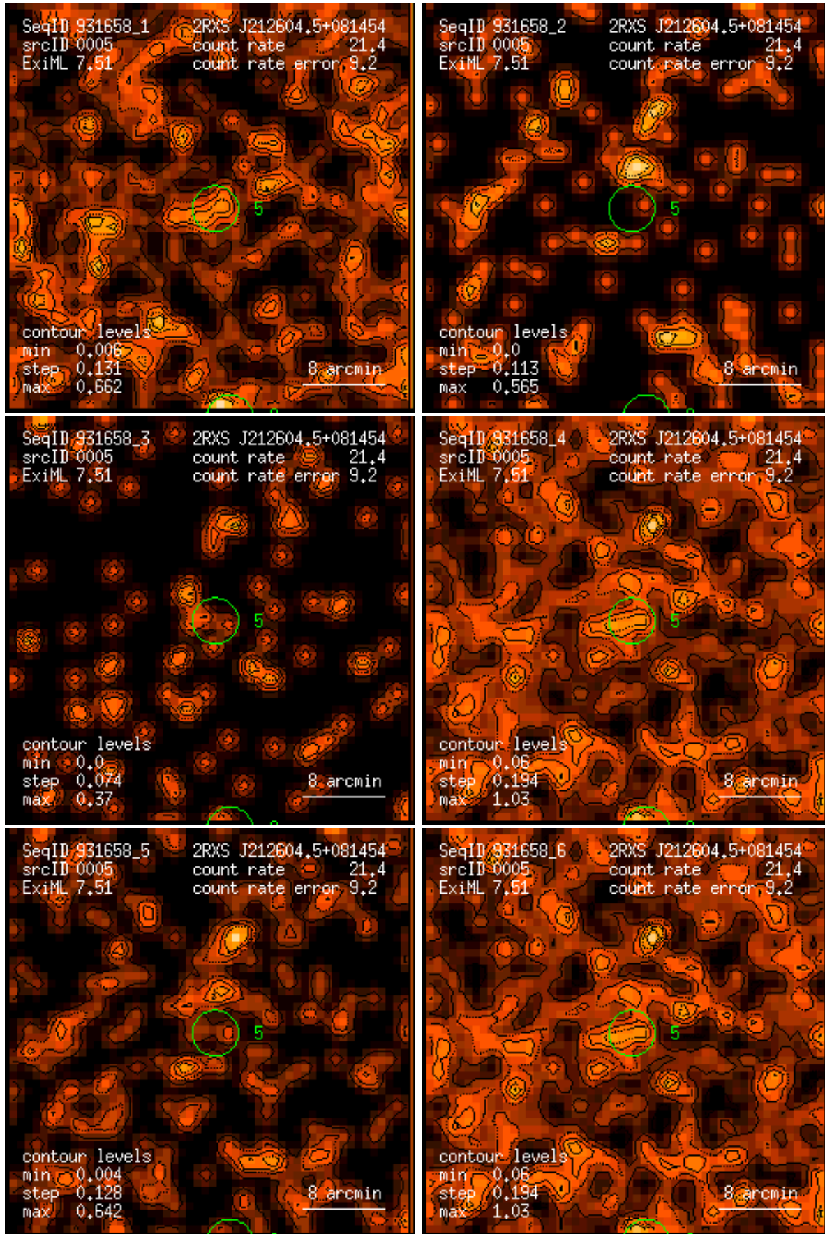
Figure 5: RASS 931658: detection 0005: band rate images, Gaussian filter: (1) PSPC channels 11 – 41, (2) 52 – 90, (3) 91 – 201, (4) 11 – 235, (5) 52 – 201, (6) 11 – 201. Broad band rates in counts/ks. Band rate contour levels in counts/ks/arcmin 2 .
