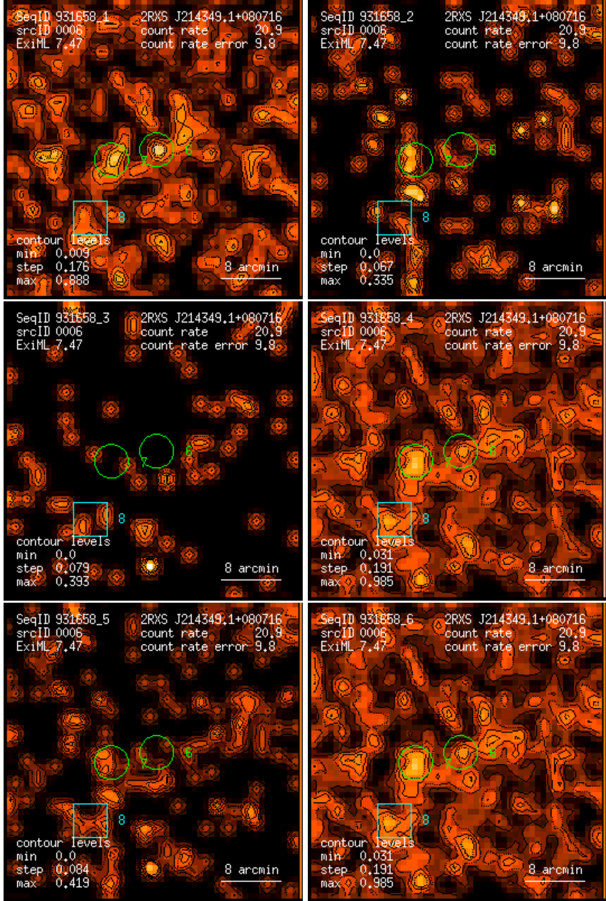
Figure 6: RASS 931658: detection 0006: band rate images, Gaussian filter: (1) PSPC channels 11 – 41, (2) 52 – 90, (3) 91 – 201, (4) 11 – 235, (5) 52 – 201, (6) 11 – 201. Broad band rates in counts/ks. Band rate contour levels in counts/ks/arcmin 2 .
