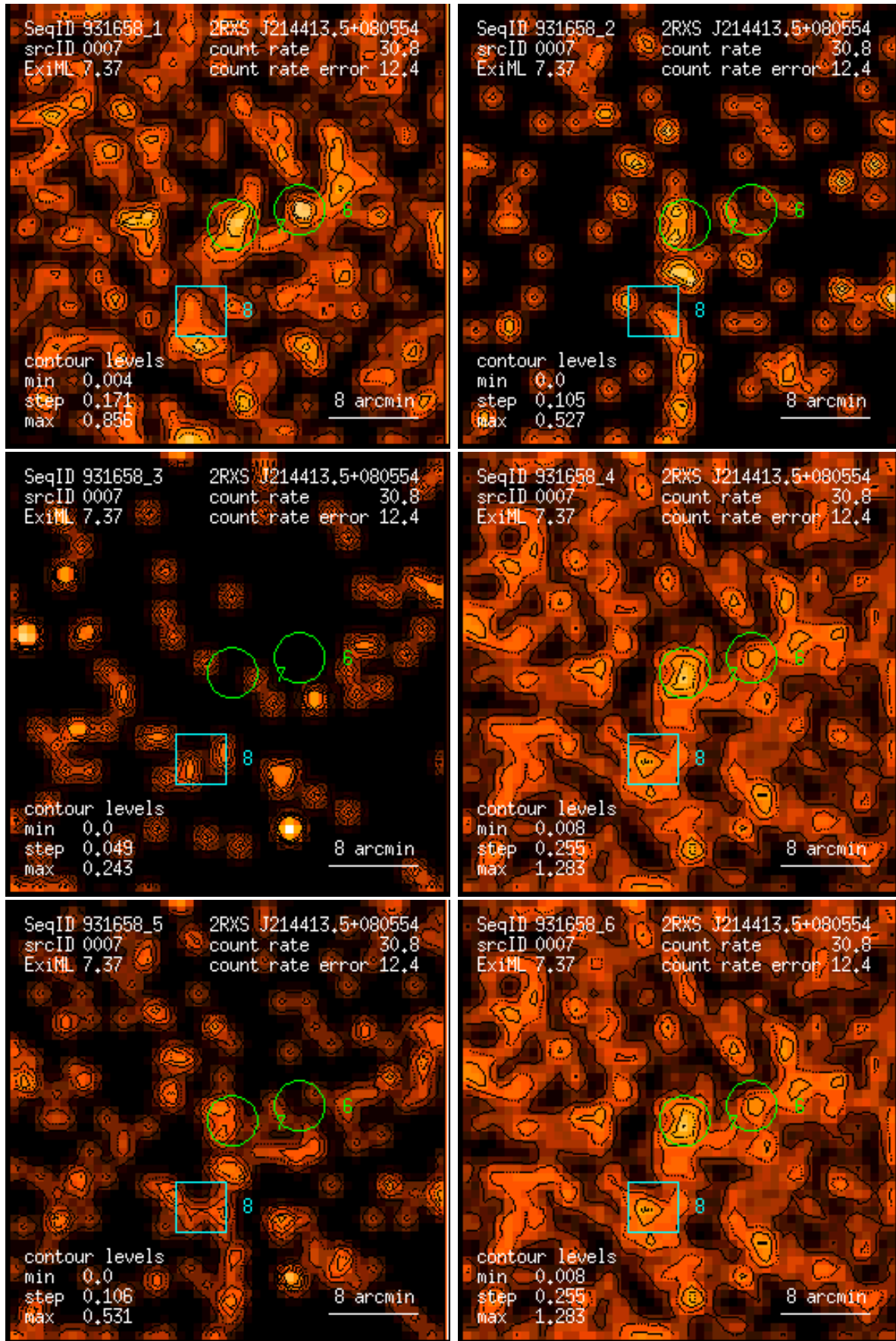
Figure 7: RASS 931658: detection 0007: band rate images, Gaussian filter: (1) PSPC channels 11 – 41, (2) 52 – 90, (3) 91 – 201, (4) 11 – 235, (5) 52 – 201, (6) 11 – 201. Broad band rates in counts/ks. Band rate contour levels in counts/ks/arcmin 2 .
