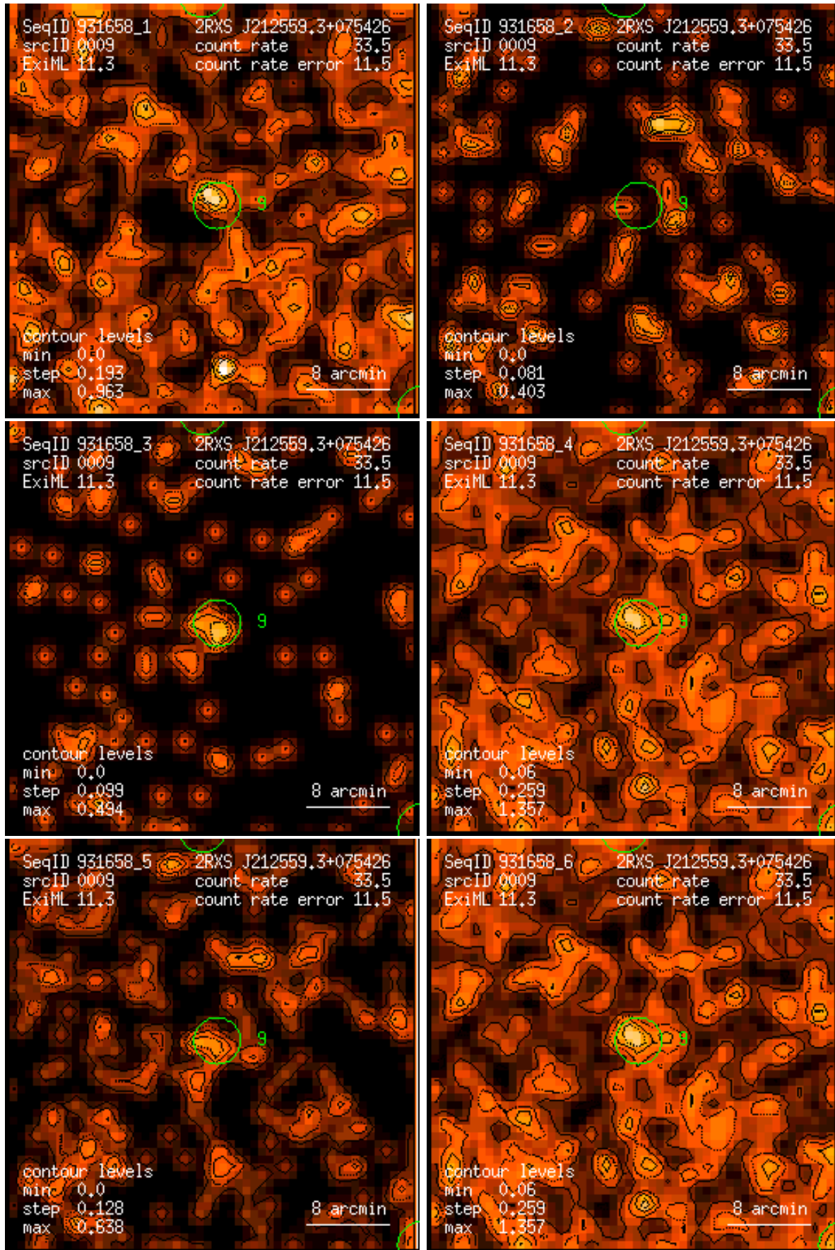
Figure 9: RASS 931658: detection 0009: band rate images, Gaussian filter: (1) PSPC channels 11 – 41, (2) 52 – 90, (3) 91 – 201, (4) 11 – 235, (5) 52 – 201, (6) 11 – 201. Broad band rates in counts/ks. Band rate contour levels in counts/ks/arcmin 2 .
