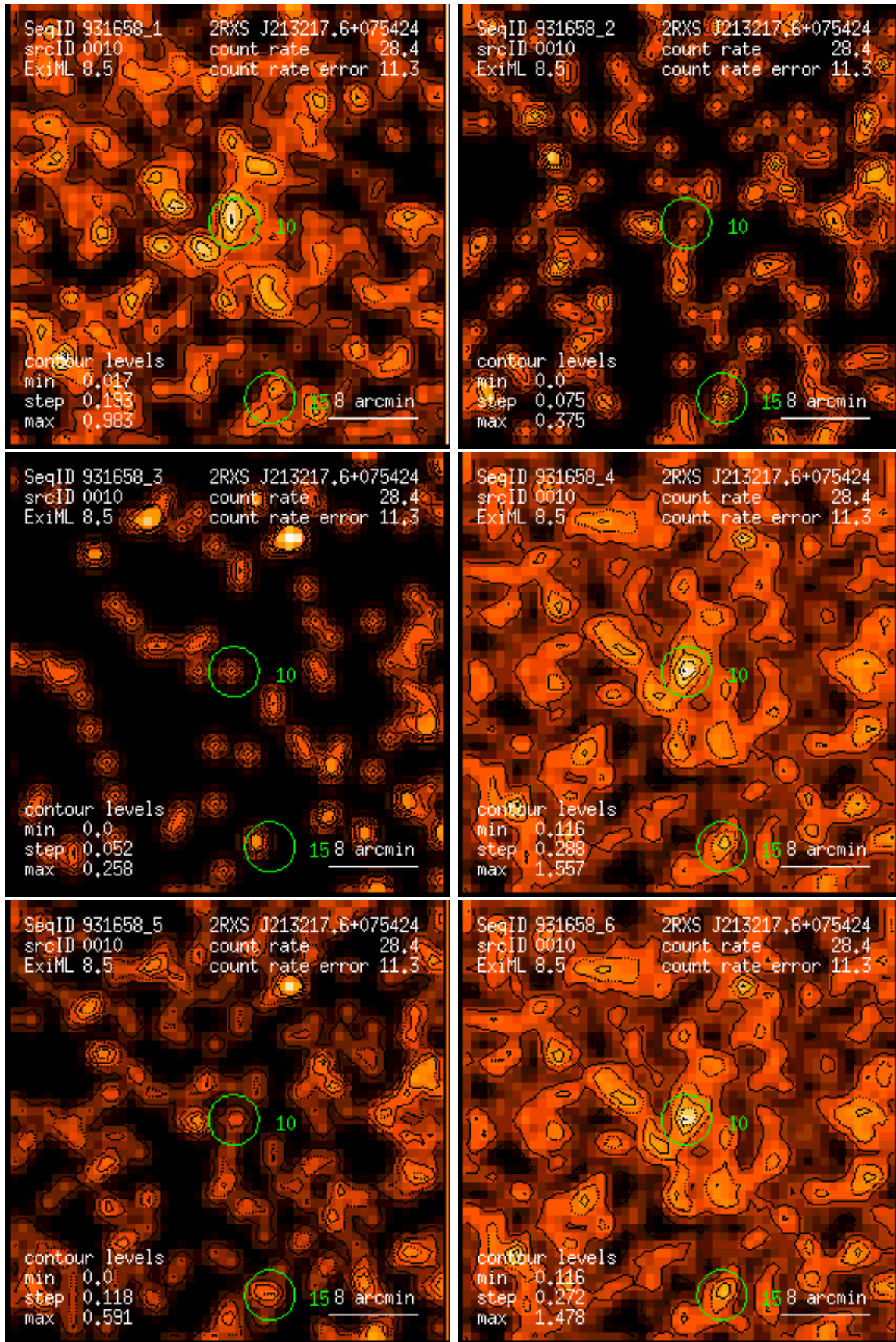
Figure 10: RASS 931658: detection 0010: band rate images, Gaussian filter: (1) PSPC channels 11 – 41, (2) 52 – 90, (3) 91 – 201, (4) 11 – 235, (5) 52 – 201, (6) 11 – 201. Broad band rates in counts/ks. Band rate contour levels in counts/ks/arcmin 2 .
