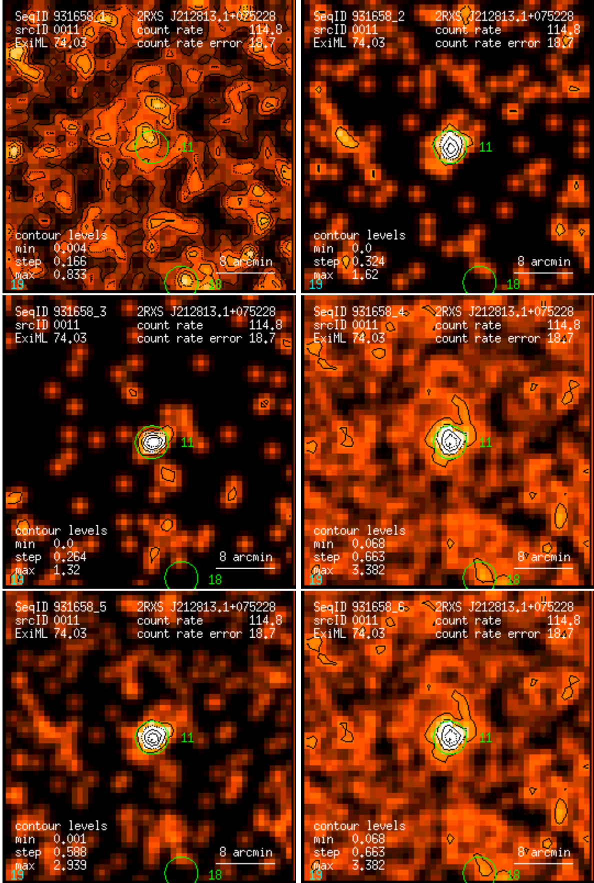
Figure 11: RASS 931658: detection 0011: band rate images, Gaussian filter: (1) PSPC channels 11 – 41, (2) 52 – 90, (3) 91 – 201, (4) 11 – 235, (5) 52 – 201, (6) 11 – 201. Broad band rates in counts/ks. Band rate contour levels in counts/ks/arcmin 2 .
