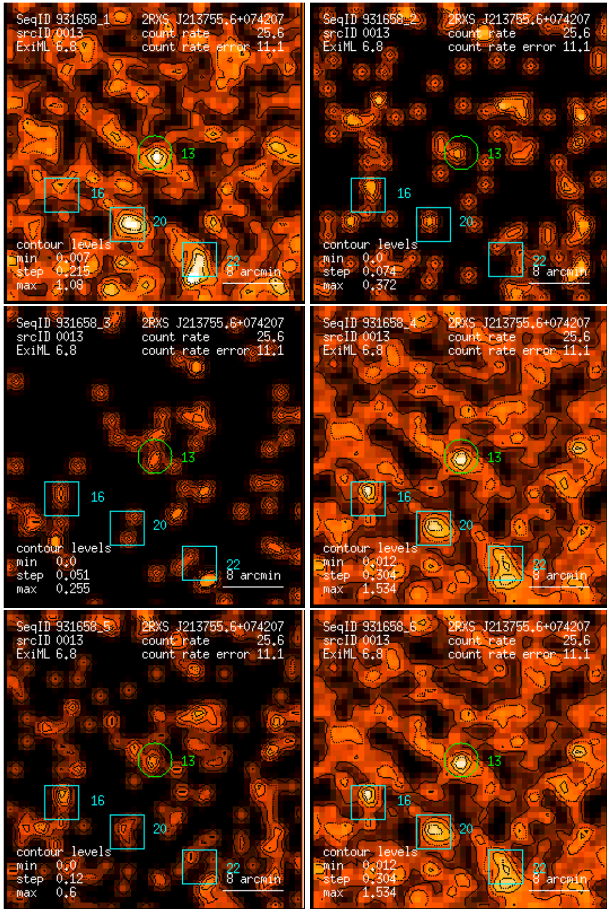
Figure 13: RASS 931658: detection 0013: band rate images, Gaussian filter: (1) PSPC channels 11 – 41, (2) 52 – 90, (3) 91 – 201, (4) 11 – 235, (5) 52 – 201, (6) 11 – 201. Broad band rates in counts/ks. Band rate contour levels in counts/ks/arcmin 2 .
