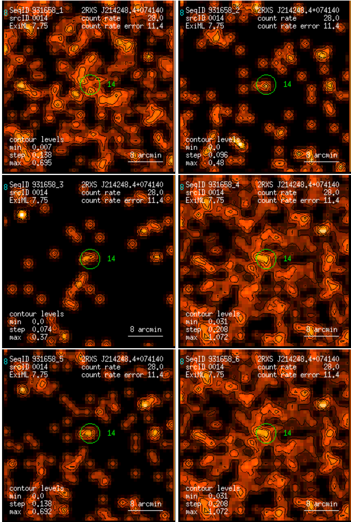
Figure 14: RASS 931658: detection 0014: band rate images, Gaussian filter: (1) PSPC channels 11 – 41, (2) 52 – 90, (3) 91 – 201, (4) 11 – 235, (5) 52 – 201, (6) 11 – 201. Broad band rates in counts/ks. Band rate contour levels in counts/ks/arcmin 2 .
