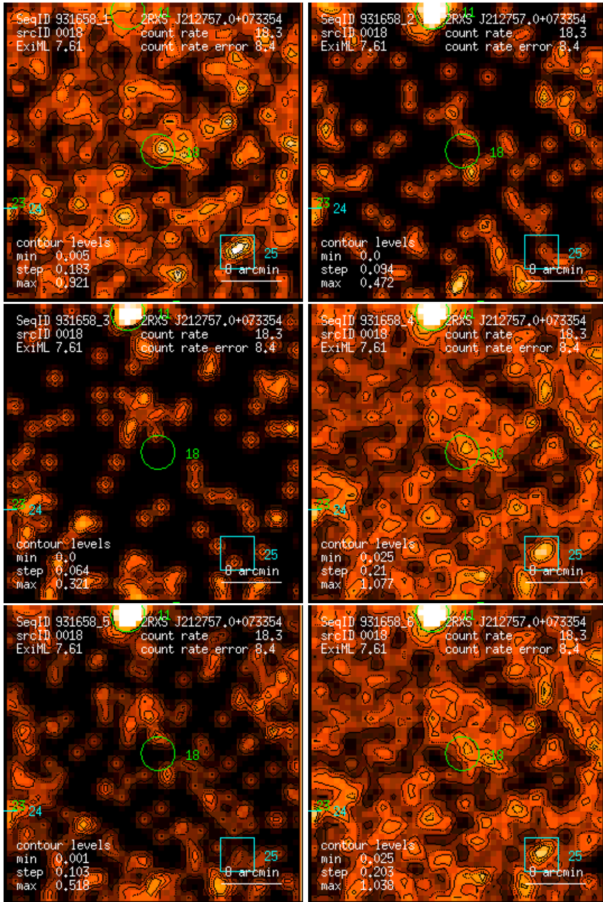
Figure 18: RASS 931658: detection 0018: band rate images, Gaussian filter: (1) PSPC channels 11 – 41, (2) 52 – 90, (3) 91 – 201, (4) 11 – 235, (5) 52 – 201, (6) 11 – 201. Broad band rates in counts/ks. Band rate contour levels in counts/ks/arcmin 2 .
