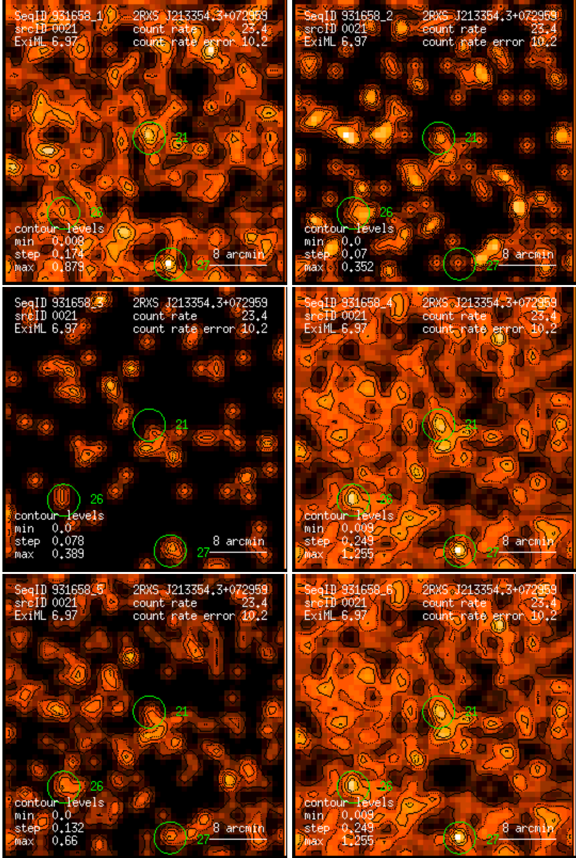
Figure 21: RASS 931658: detection 0021: band rate images, Gaussian filter: (1) PSPC channels 11 – 41, (2) 52 – 90, (3) 91 – 201, (4) 11 – 235, (5) 52 – 201, (6) 11 – 201. Broad band rates in counts/ks. Band rate contour levels in counts/ks/arcmin 2 .
