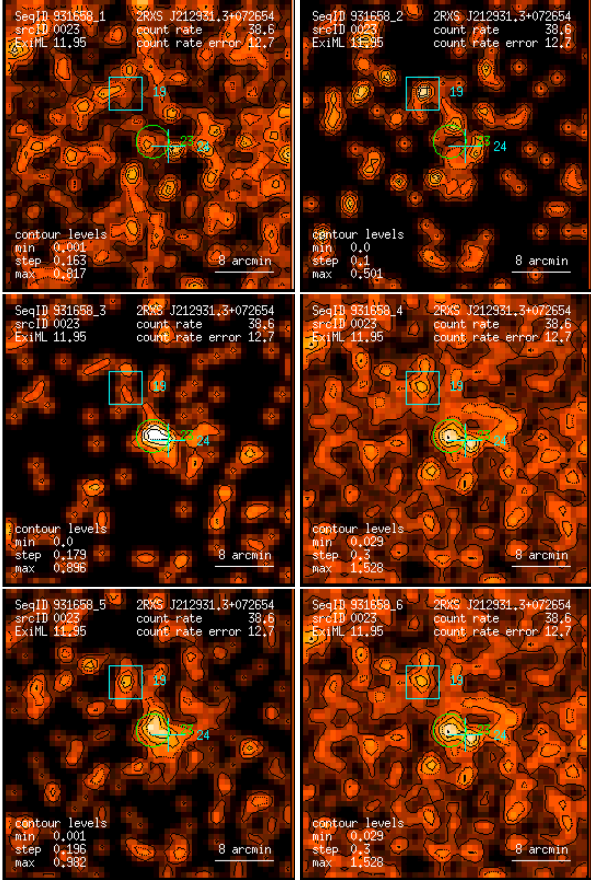
Figure 23: RASS 931658: detection 0023: band rate images, Gaussian filter: (1) PSPC channels 11 – 41, (2) 52 – 90, (3) 91 – 201, (4) 11 – 235, (5) 52 – 201, (6) 11 – 201. Broad band rates in counts/ks. Band rate contour levels in counts/ks/arcmin 2 .
